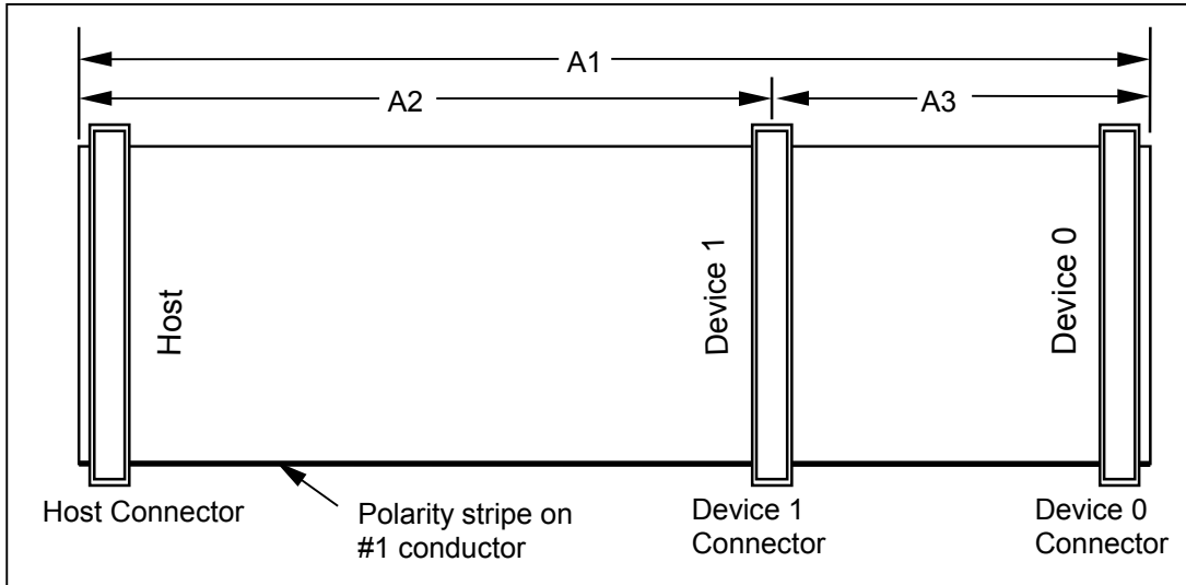
Figure 9 – 80-conductor cable configuration
