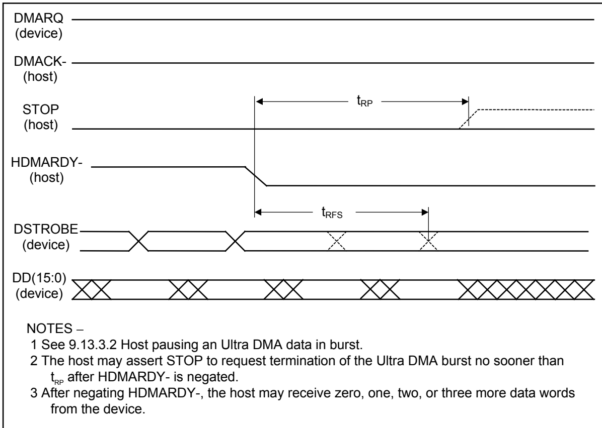
Figure 72 – Host pausing an Ultra DMA data-in burst
