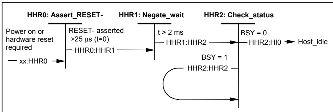
Figure 35 – Host power-on or hardware reset state diagram
