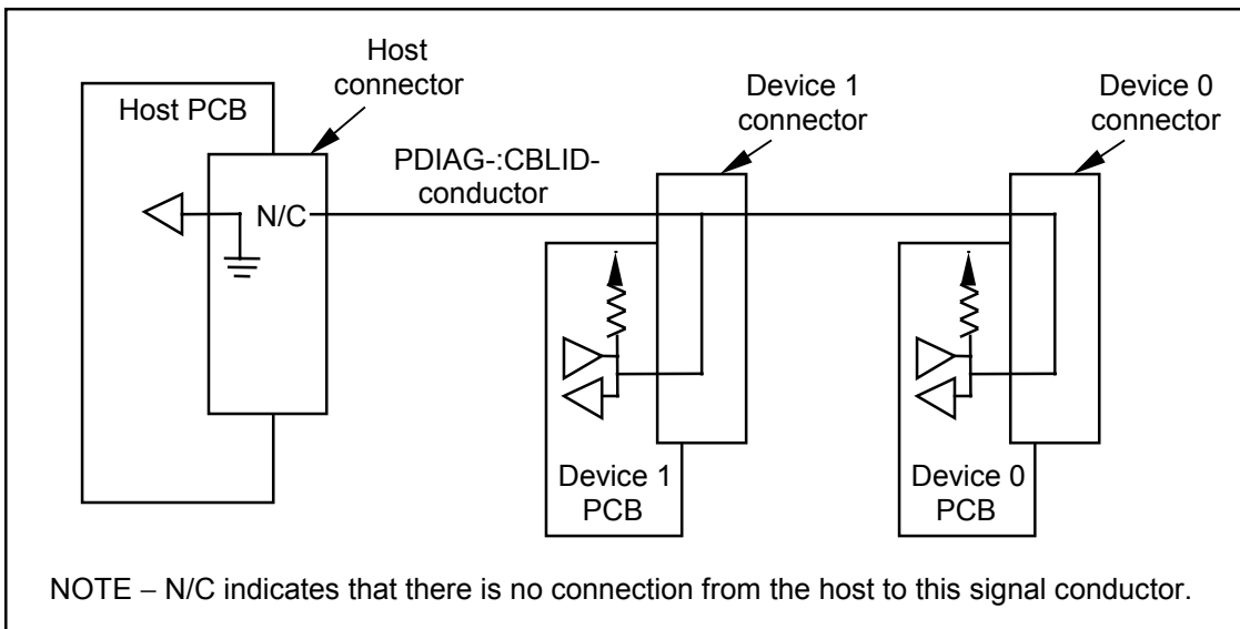
Figure 32 – Example configuration of a system where the host detects an 80-conductor cable
