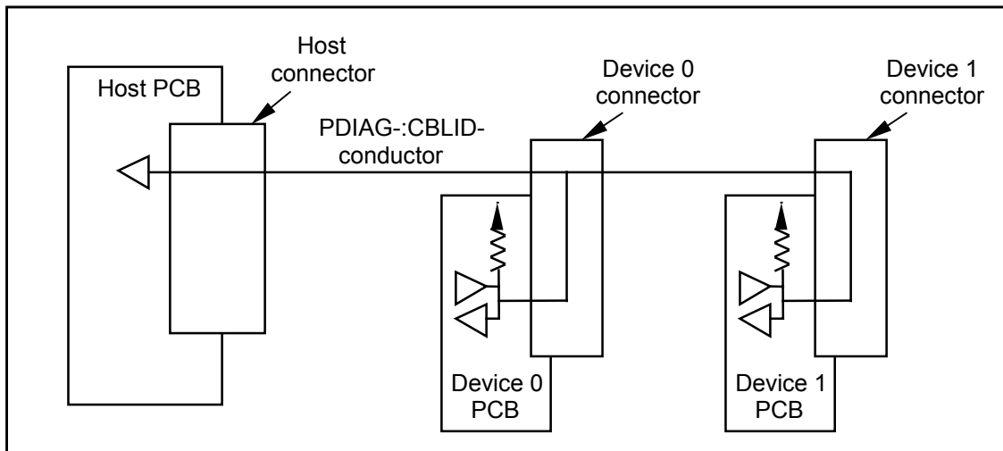
Figure 31 – Example configuration of a system where the host detects a 40-conductor cable
