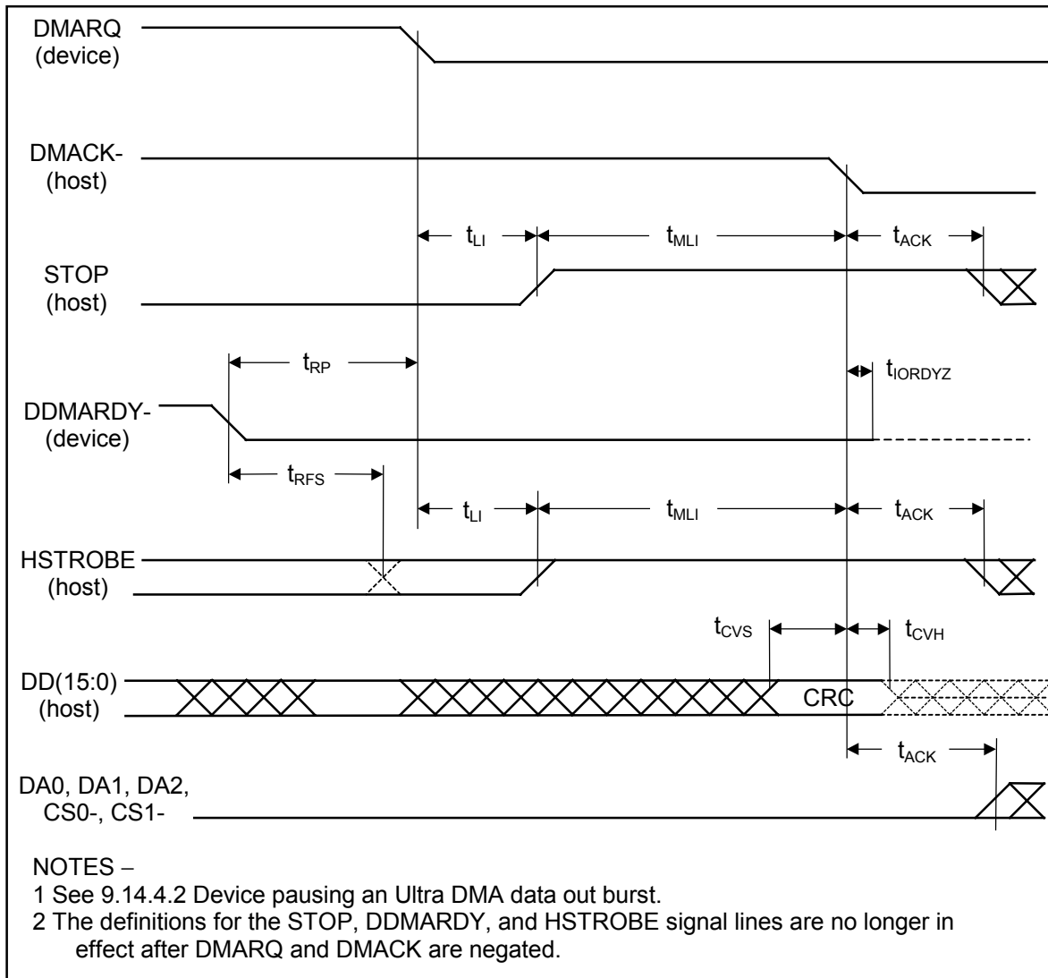
Figure 79 – Device terminating an Ultra DMA data-out burst
