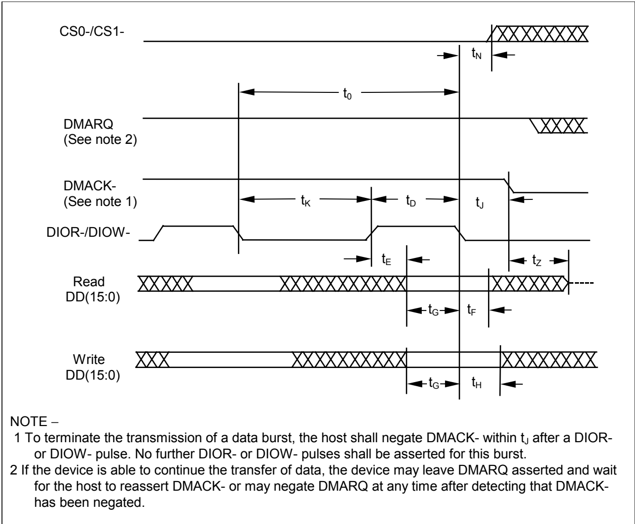
Figure 69 – Host terminating a Multiword DMA data burst
