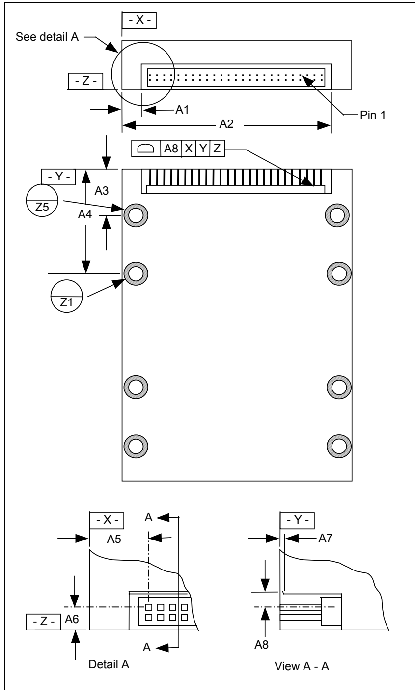
Figure 21 – 2.5" form factor connector location
