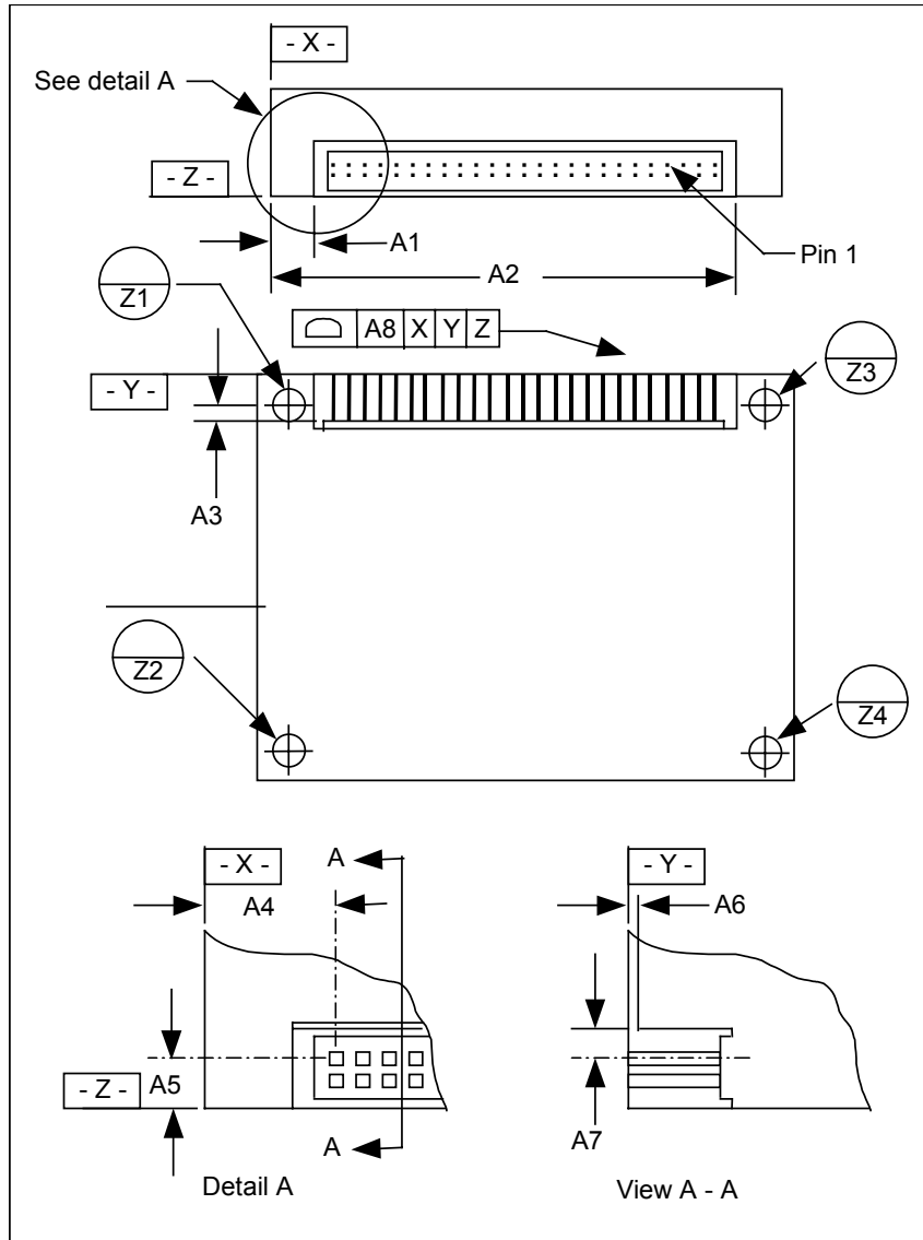
Figure 23 – 1.8 inch 5V parallel form factor connector location
