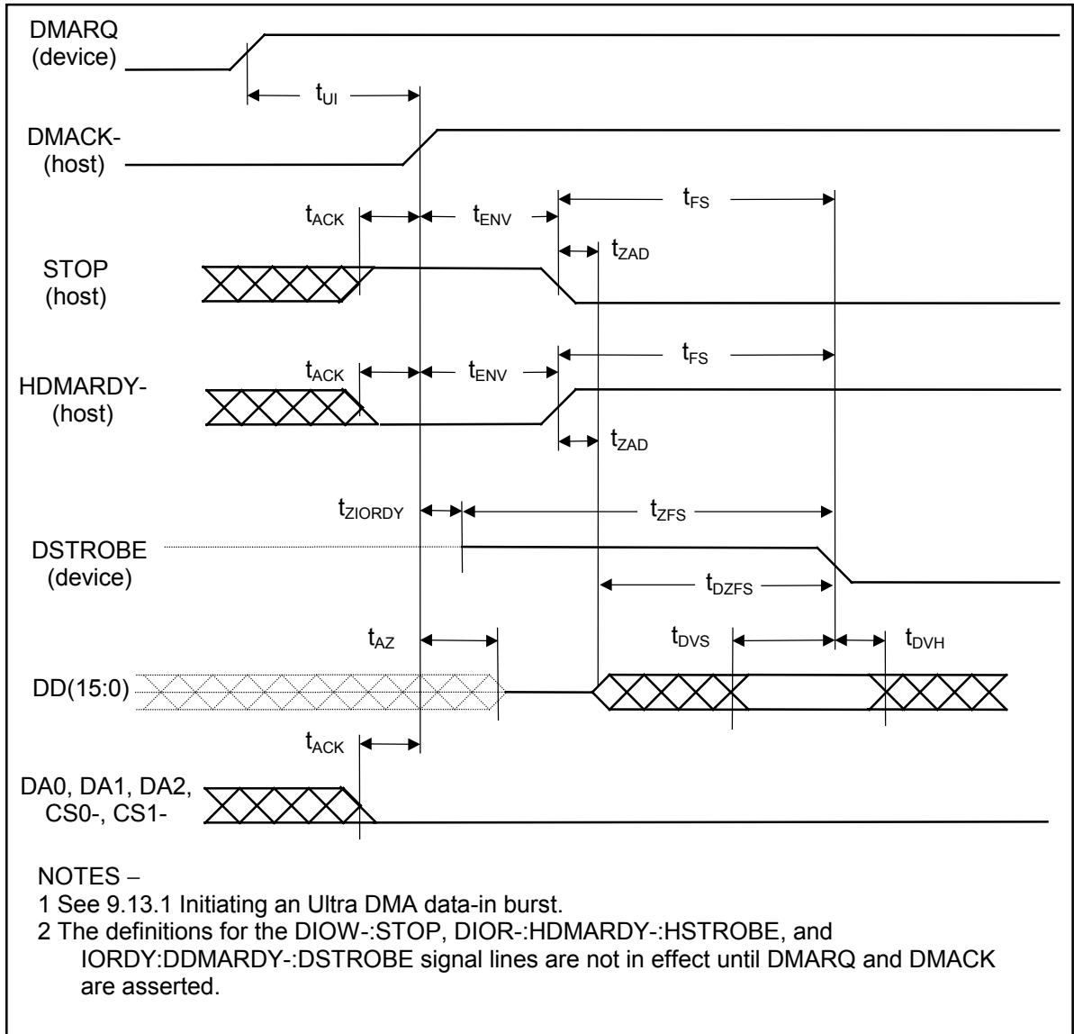
Figure 70 – Initiating an Ultra DMA data-in burst
