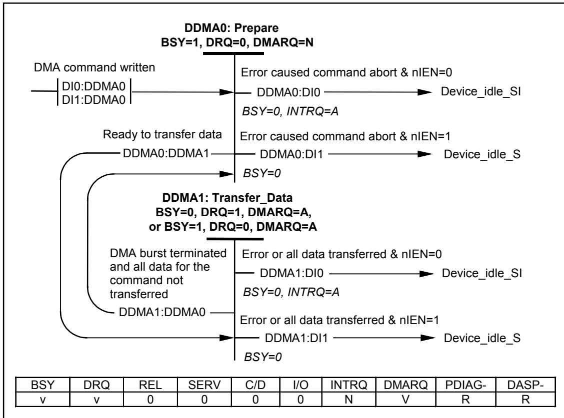
Figure 51 – Device DMA state diagram
