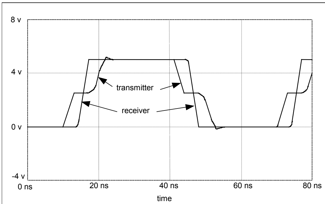
Figure E.2 – Waveforms on a source-terminated bus with rise time less than T_{prop}
