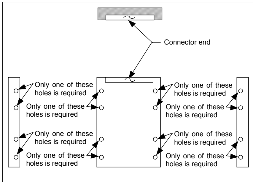
Figure 20 –2.5" form factor mounting holes
