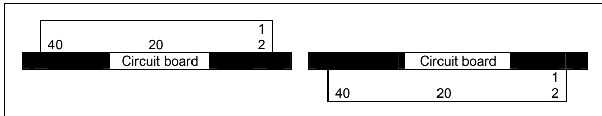
Figure 6 – 40-pin I/O header mounting
