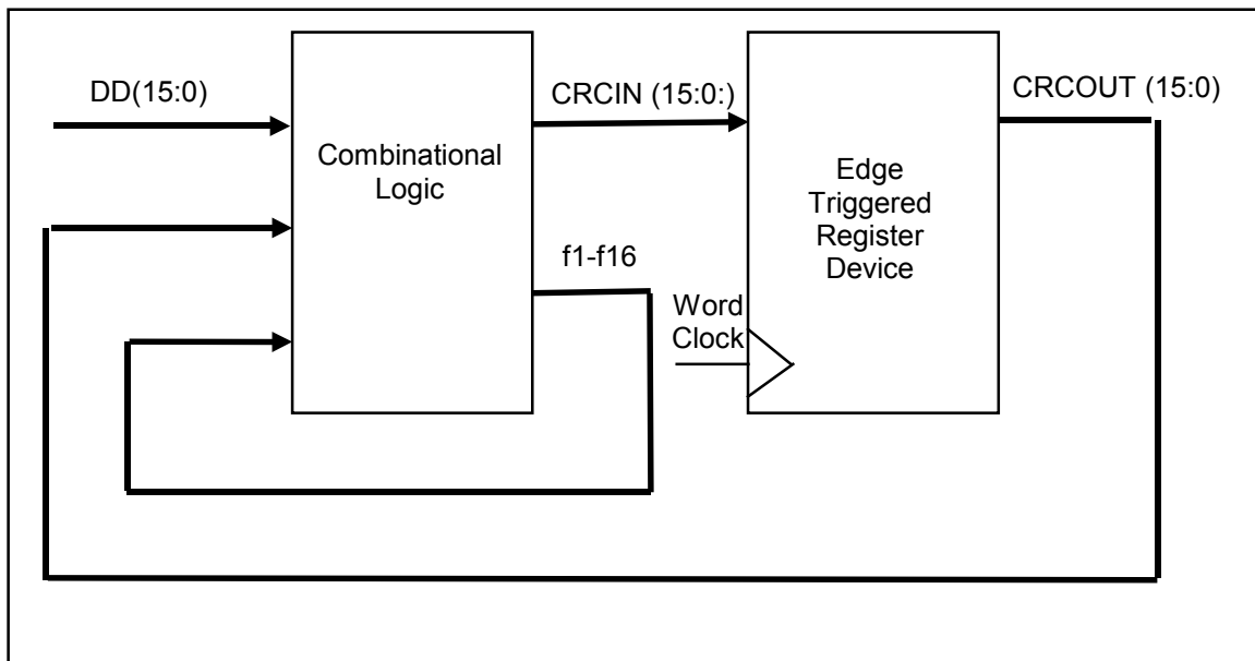
Figure 63 – Example Parallel CRC generator
