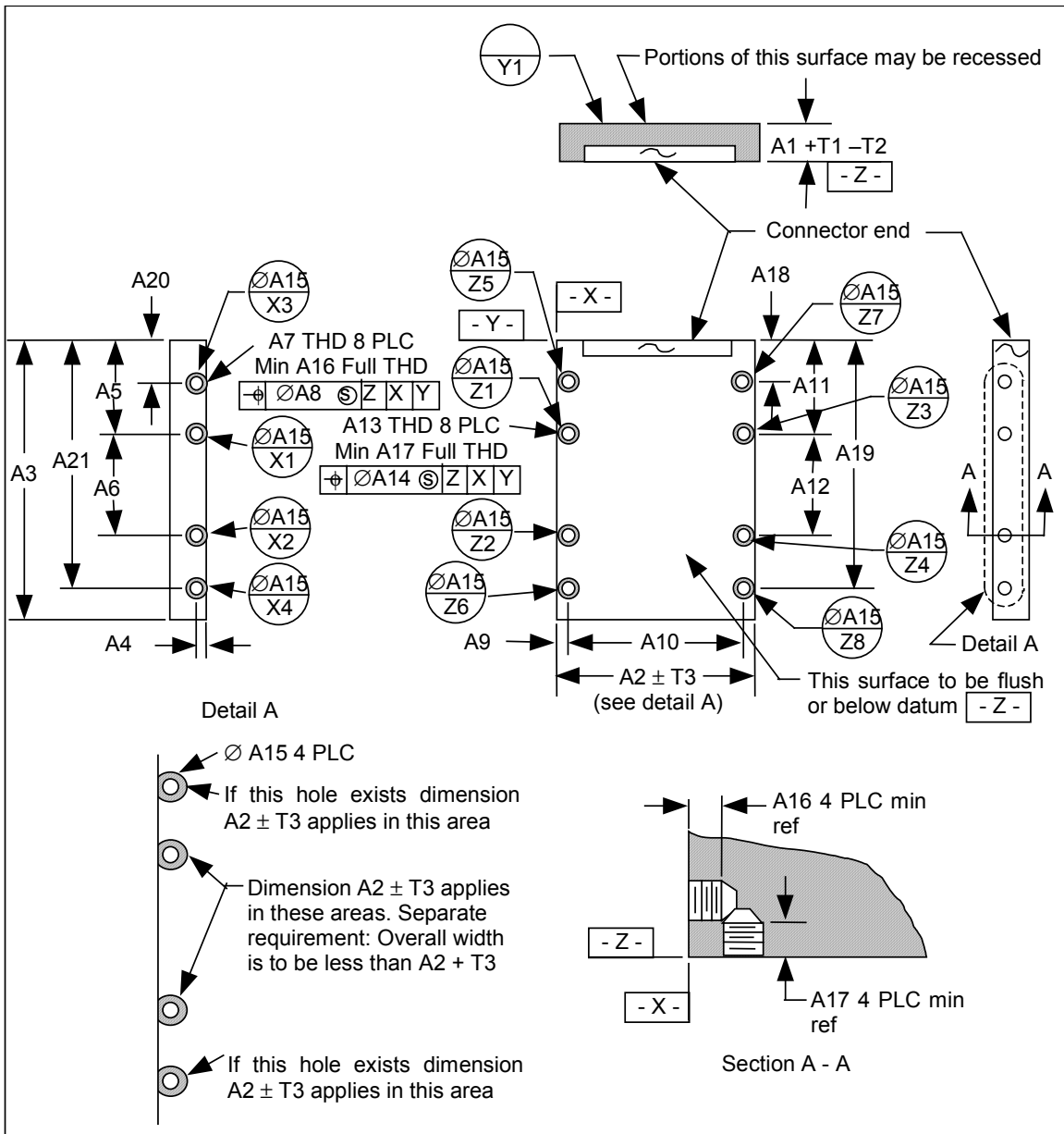
Figure 19 – 2.5" form factor
