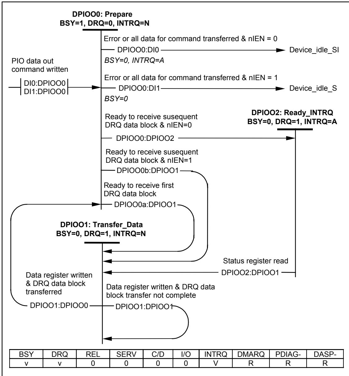
Figure 49 – Device PIO data-Out state diagram
