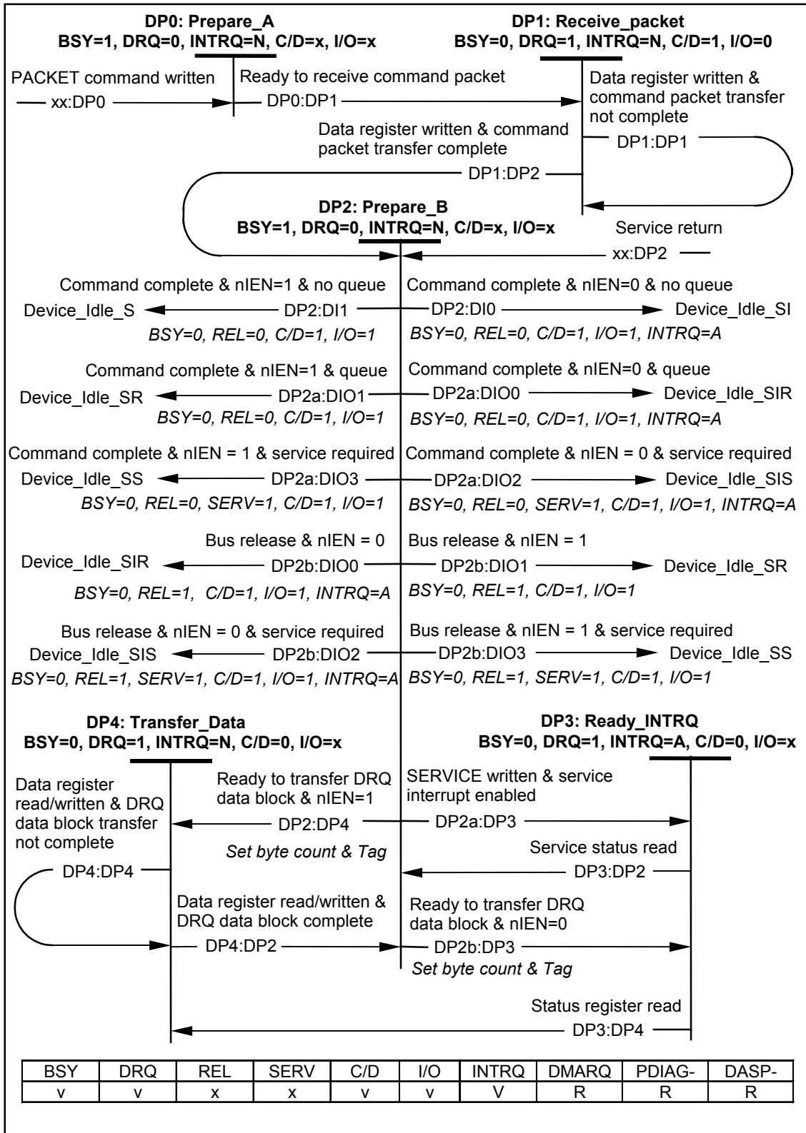
Figure 53 – Device PACKET non-data and PIO data command state diagram
