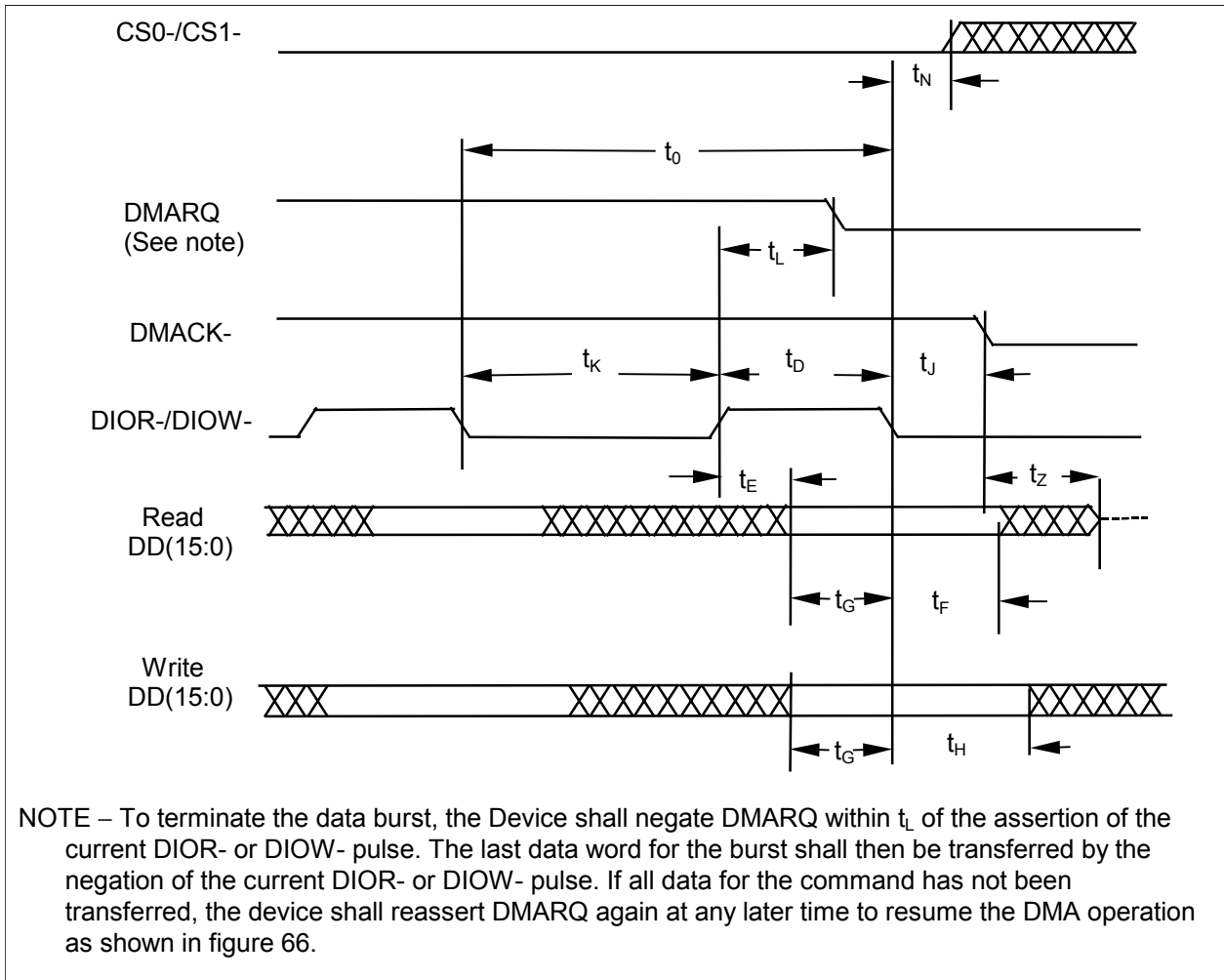
Figure 68 – Device terminating a Multiword DMA data burst
