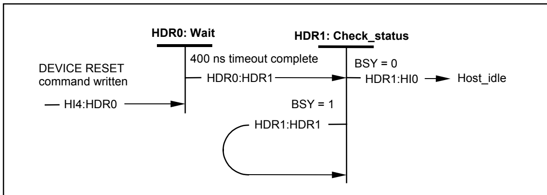
Figure 61 – Host DEVICE RESET command state diagram
