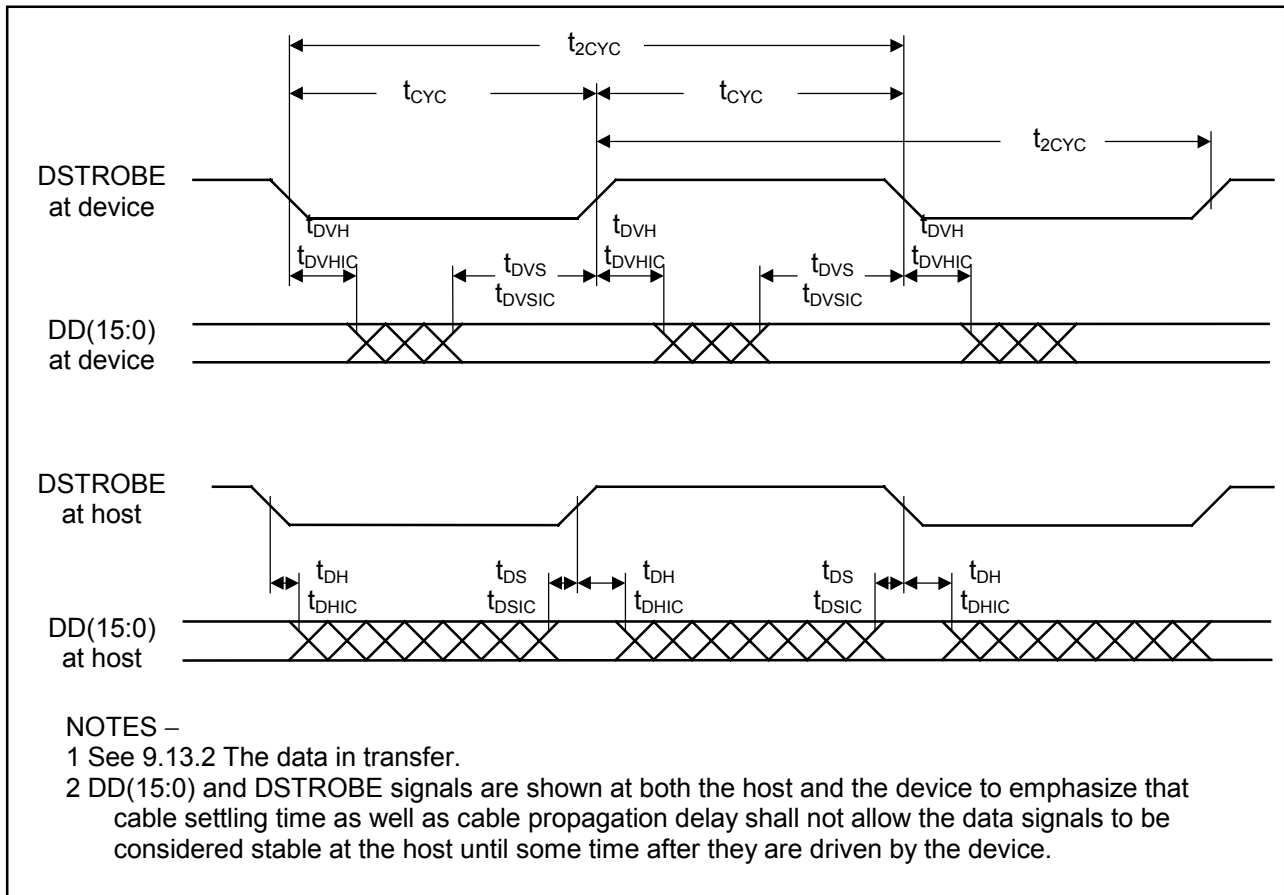
Figure 71 – Sustained Ultra DMA data-in burst
