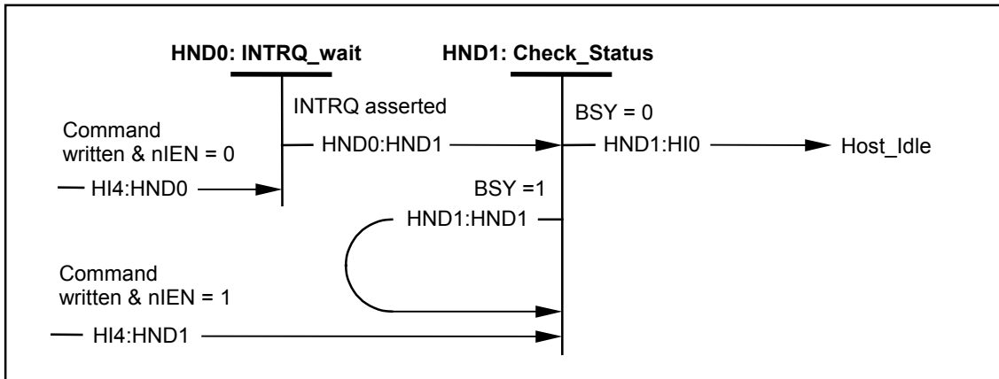
Figure 44 – Host Non-Data state diagram
