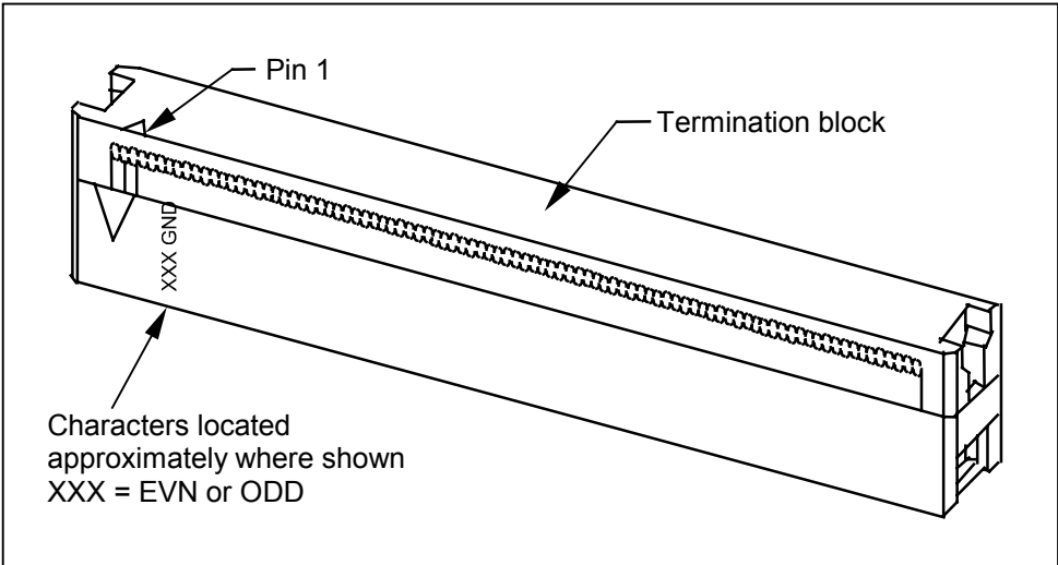
Figure 10 – Connector labeling for even or odd conductor grounding
