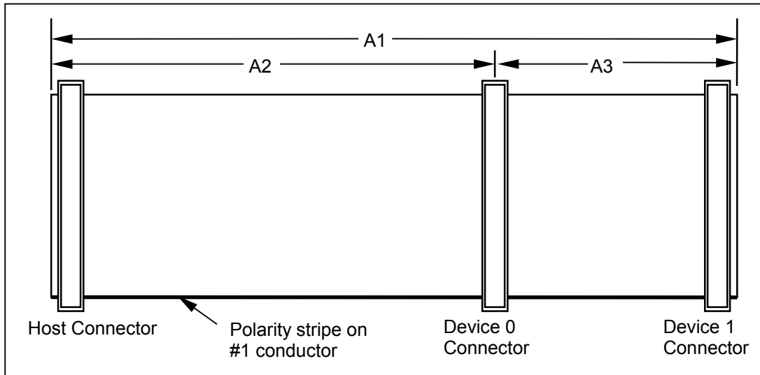
Figure 7 – 40-conductor cable configuration
