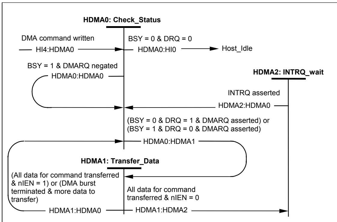
Figure 50 – Host DMA state diagram
