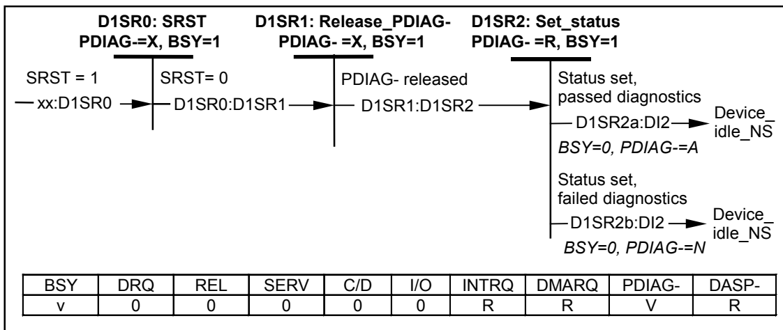
Figure 39 – Device 1 software reset state diagram
