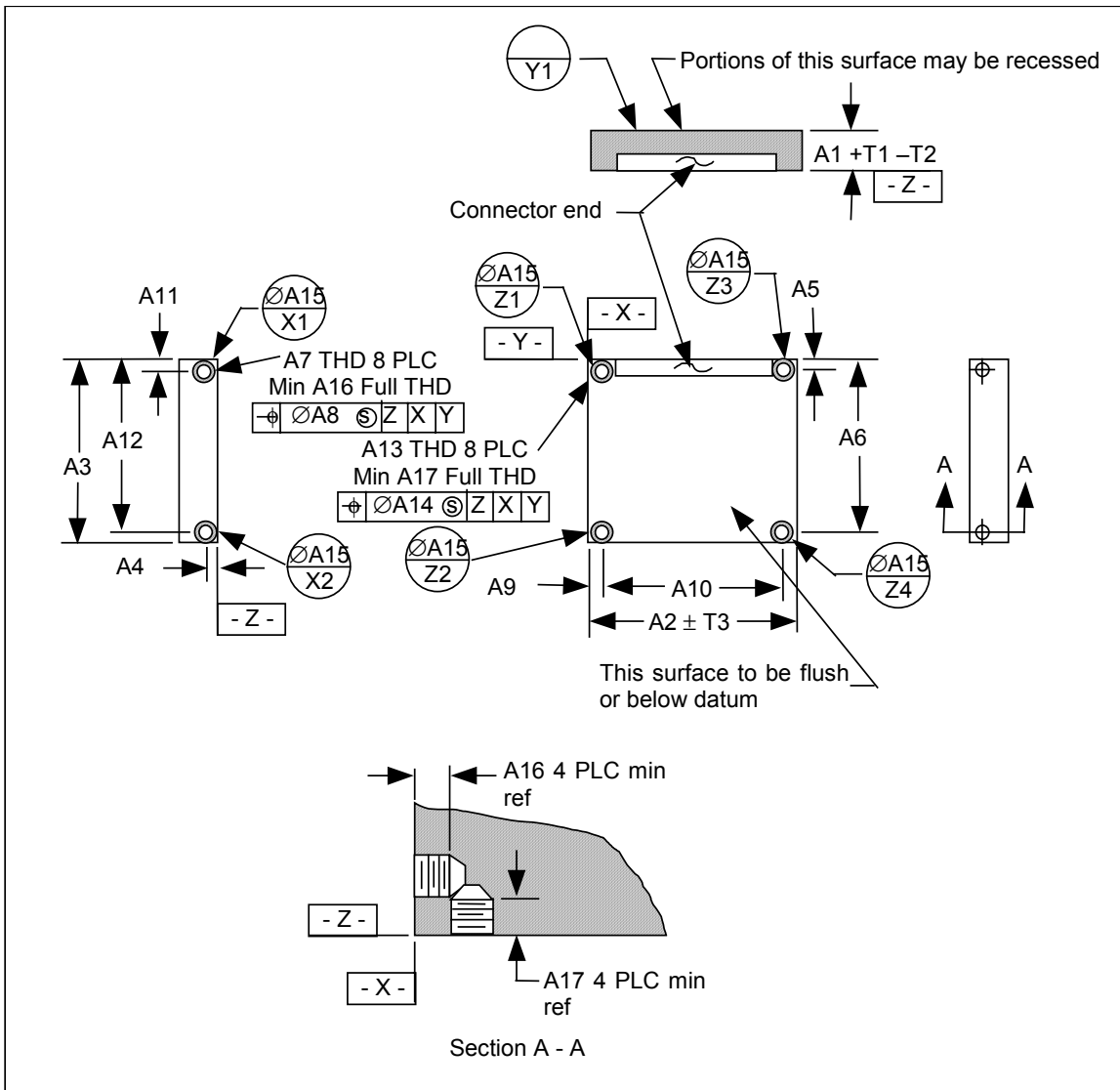
Figure 22 – 1.8 inch 5V parallel form factor
