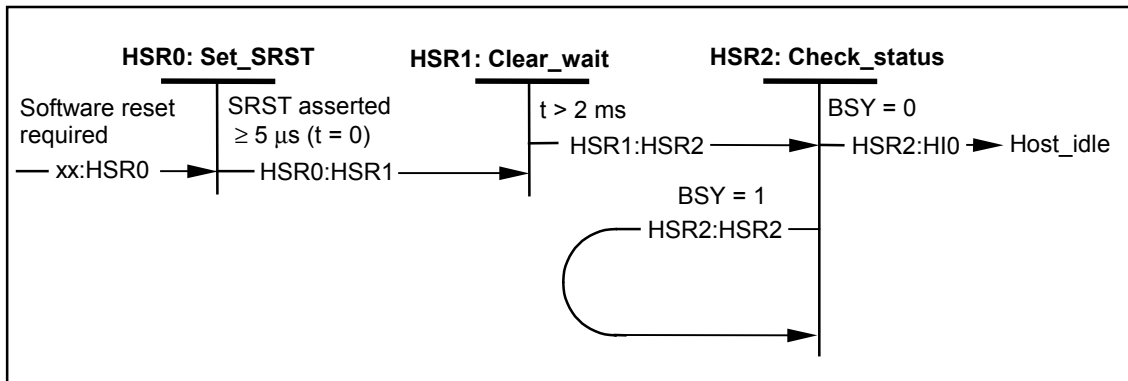
Figure 37 – Host software reset state diagram
