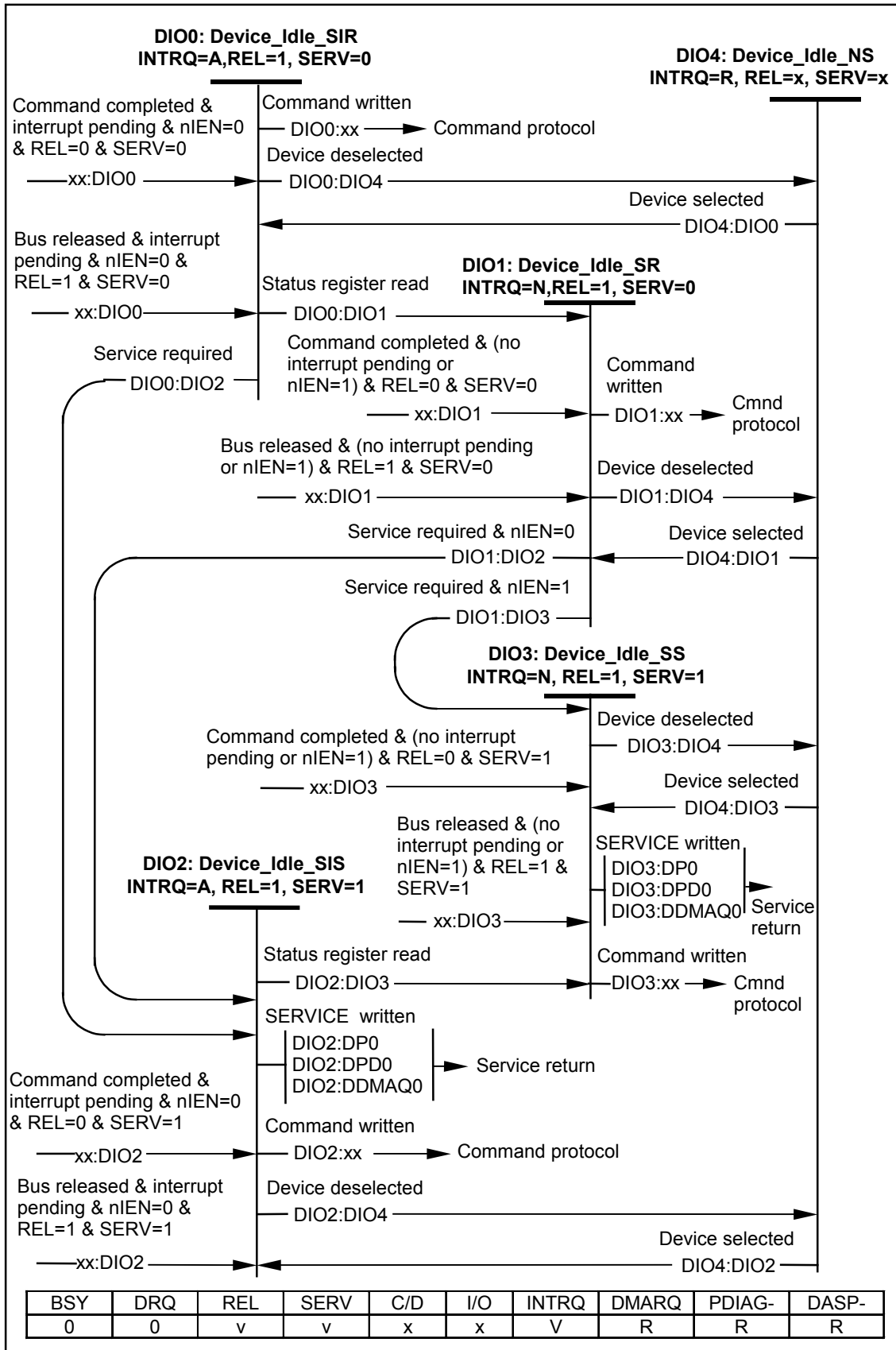
Figure 43 – Additional Device bus Idle state diagram with Overlap or overlap and queuing
