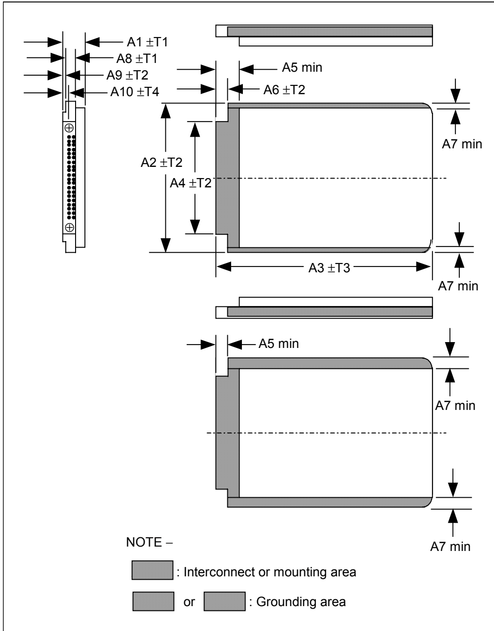
Figure 24 – 1.8 inch 3.3V parallel form factor
