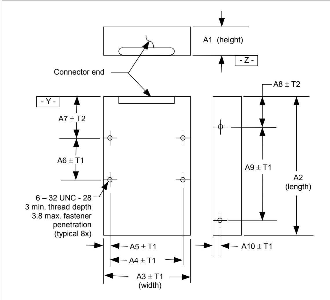
Figure 18 – 3.5" form factor
