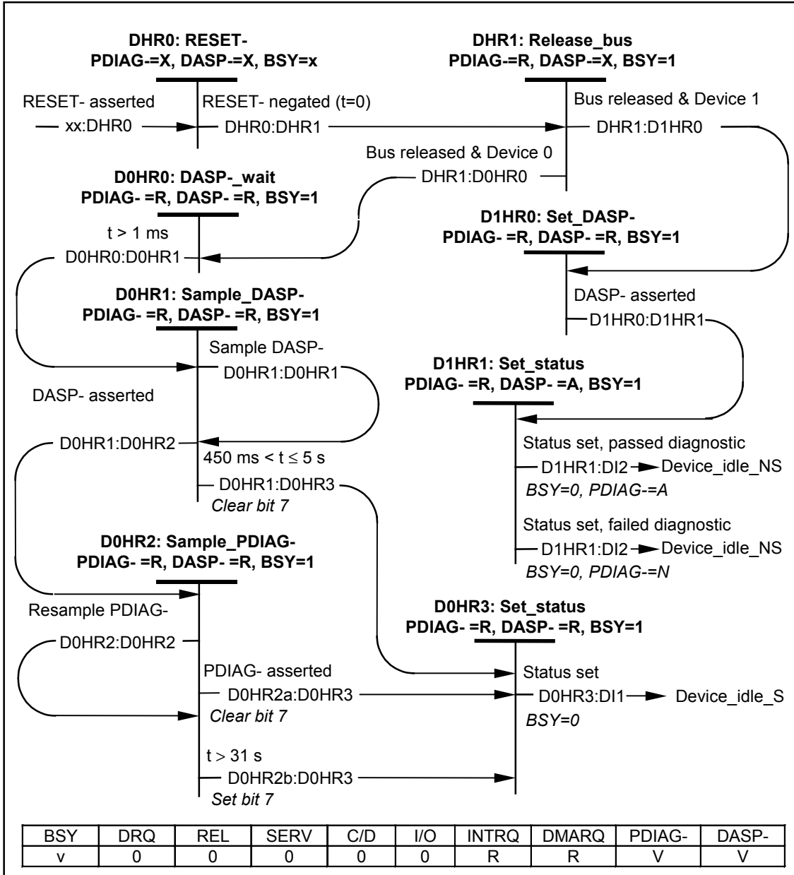
Figure 36 – Device power-on or hardware reset state diagram
