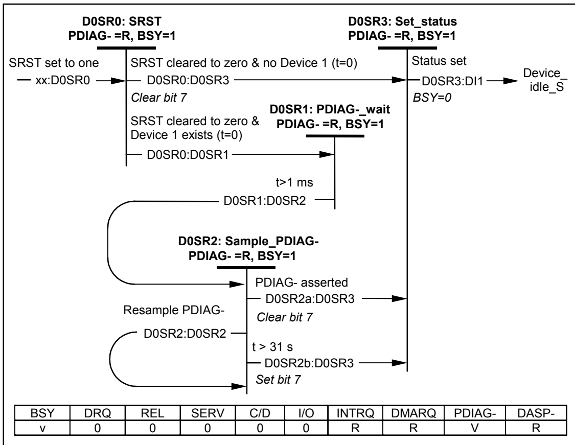
Figure 38 – Device 0 software reset state diagram
