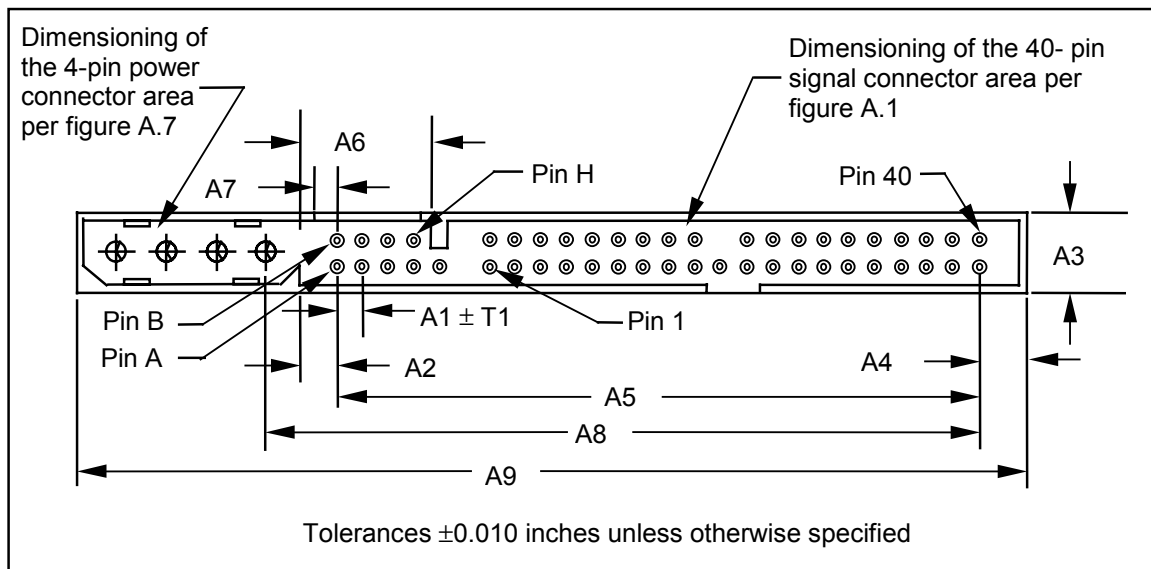
Figure 13 – Unitized connector
