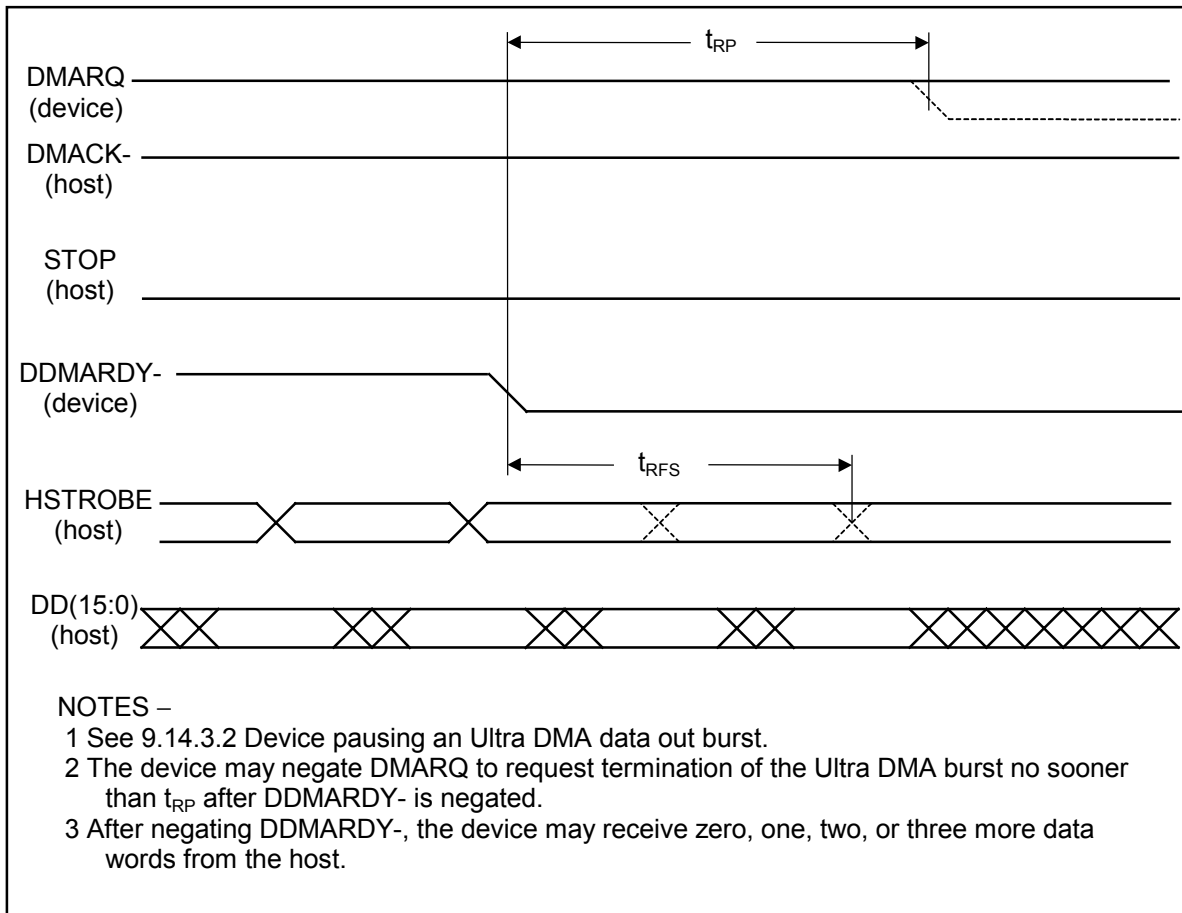
Figure 77 – Device pausing an Ultra DMA data-out burst
