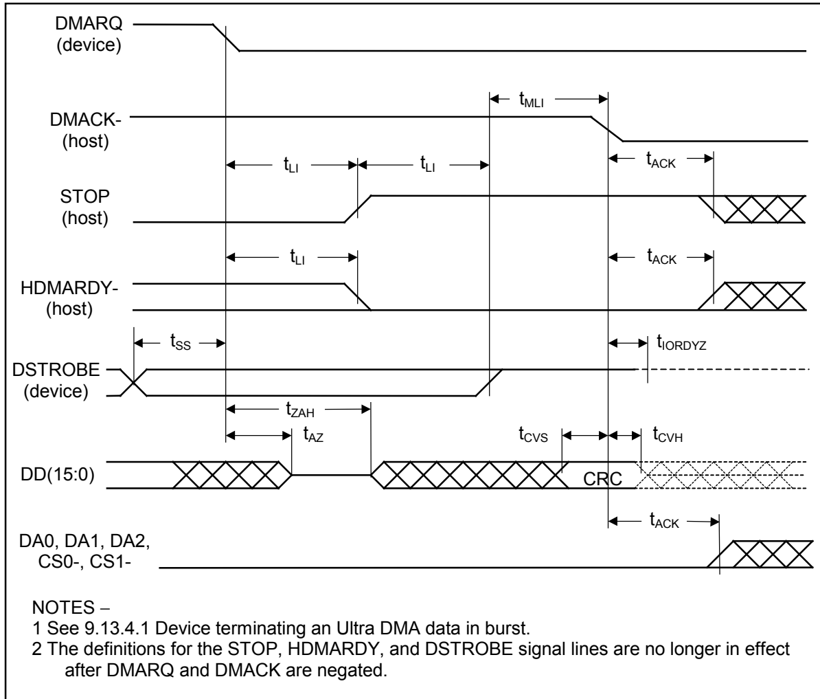
Figure 73 – Device terminating an Ultra DMA data-in burst
