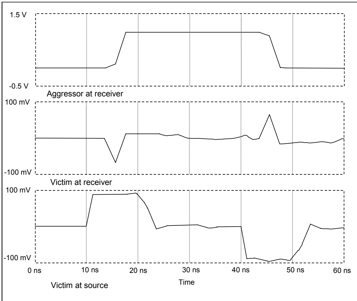
Figure E.17 – Waveforms resulting from distributed coupling (at transmitter and receiver of aggressor and victim lines)
