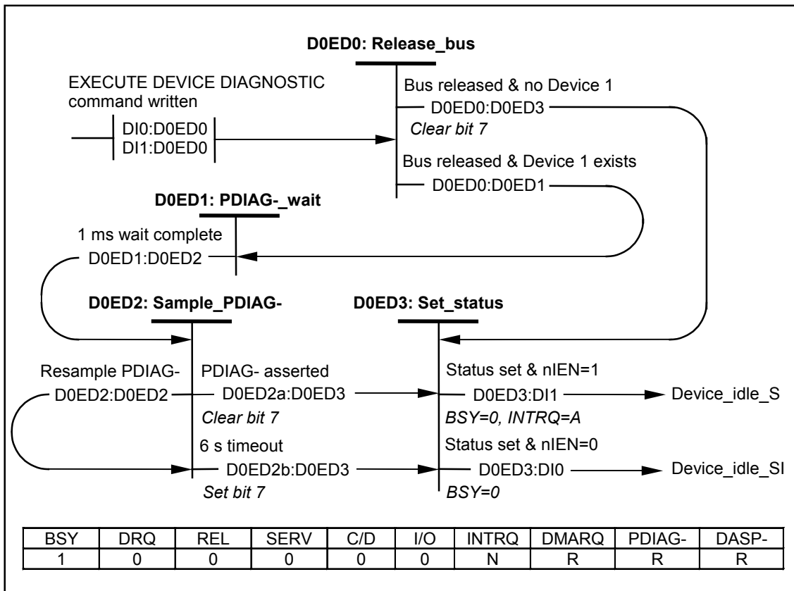
Figure 59 – Device 0 EXECUTE DEVICE DIAGNOSTIC state diagram
