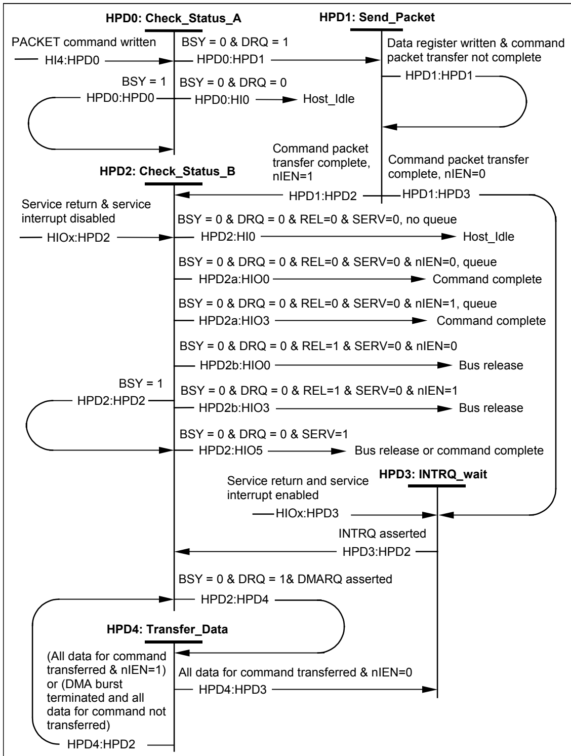
Figure 54 – Host PACKET DMA command state diagram
