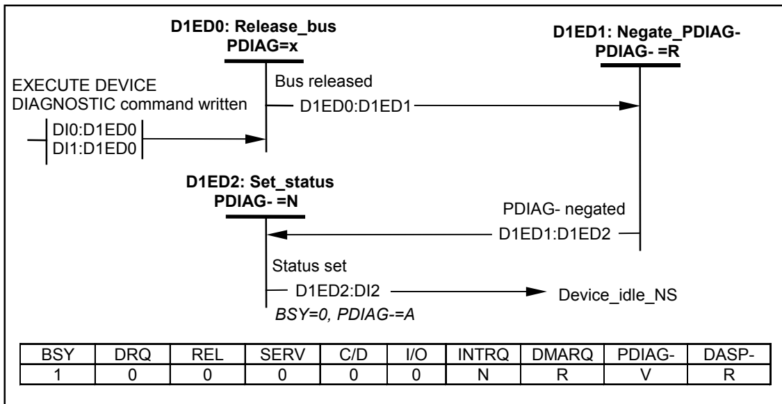
Figure 60 – Device 1 EXECUTE DEVICE DIAGNOSTIC command state diagram
