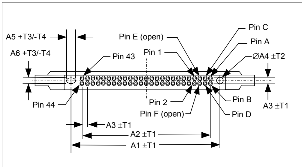
Figure 16 – 1.8 inch 3.3V parallel connector
