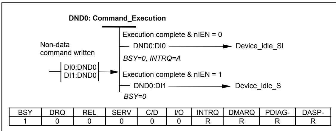
Figure 45 – Device Non-Data state diagram
