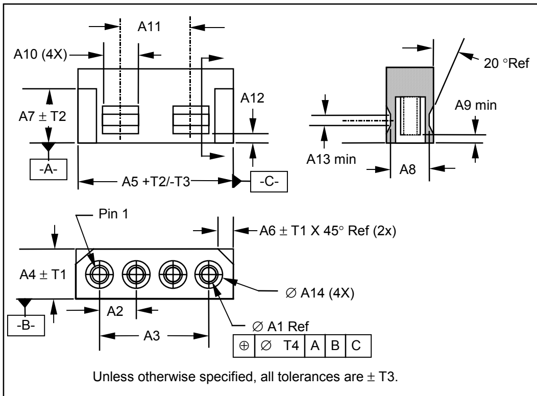
Figure 12 – 4-pin power cable connector
