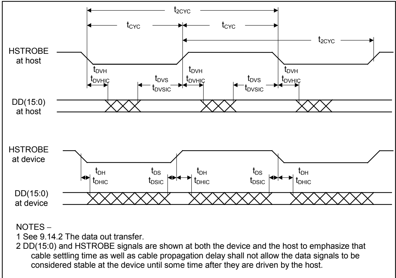
Figure 76 – Sustained Ultra DMA data-out burst
