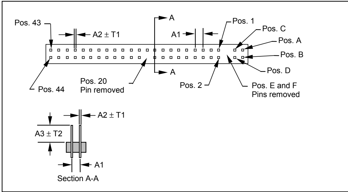
Figure 15 – 50-pin 2.5 inch form factor style connector
