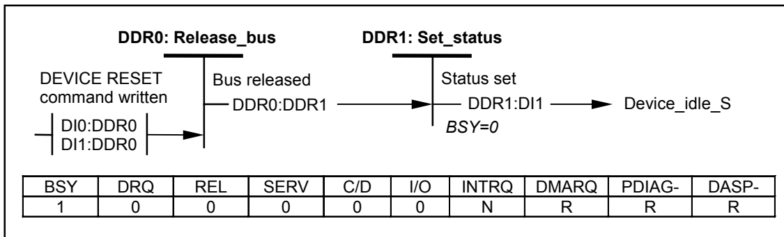
Figure 62 – Device DEVICE RESET command state diagram
