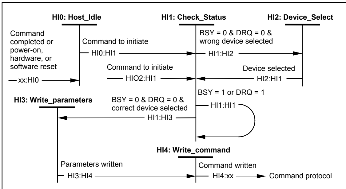
Figure 40 – Host bus idle state diagram
