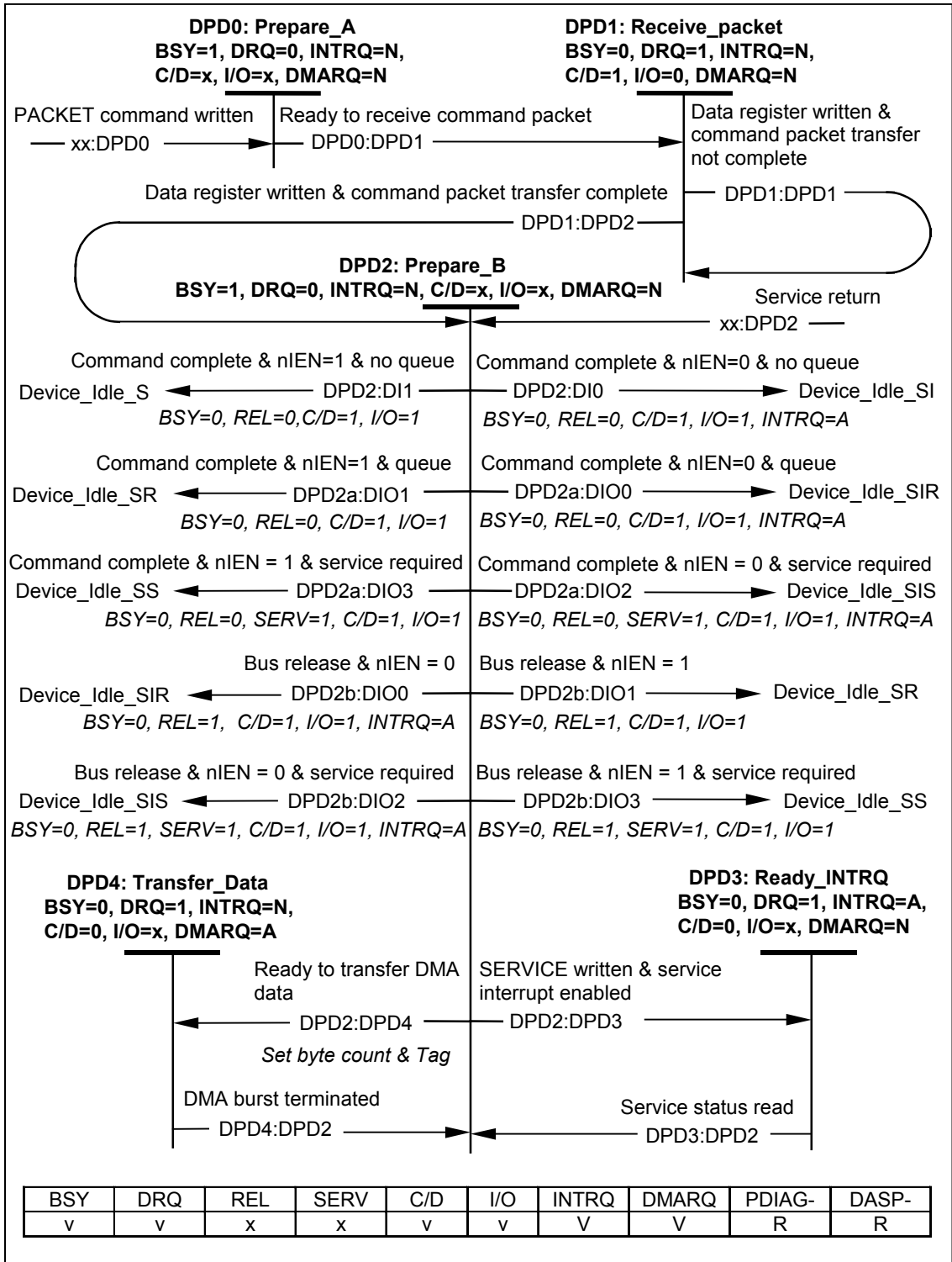
Figure 55 – Device PACKET DMA command state diagram
