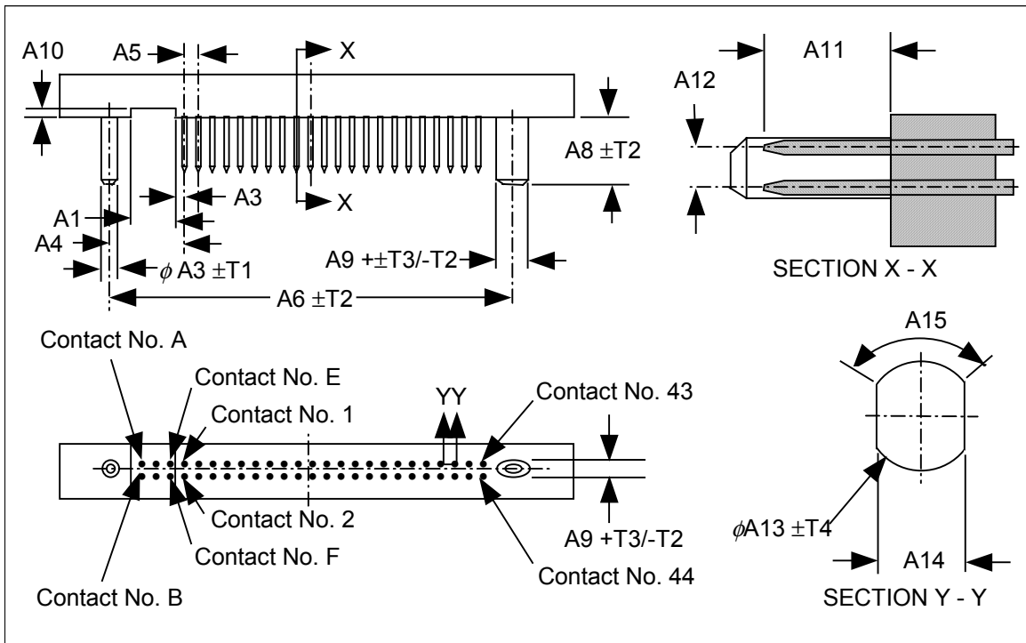
Figure 17 – 1.8 inch 3.3 V parallel host connector
