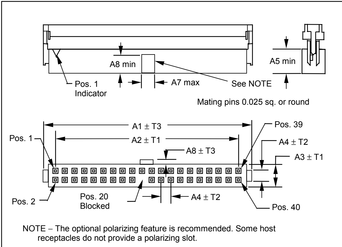
Figure 5 – 40-pin I/O cable connector
