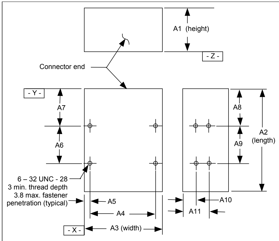
Figure 25 – 5.25 inch HDD form factor
