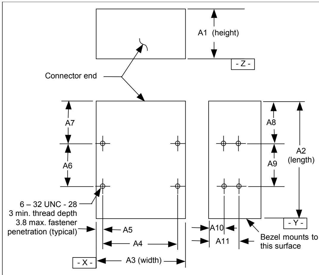
Figure 26 – 5.25 inch CD-ROM form factor
