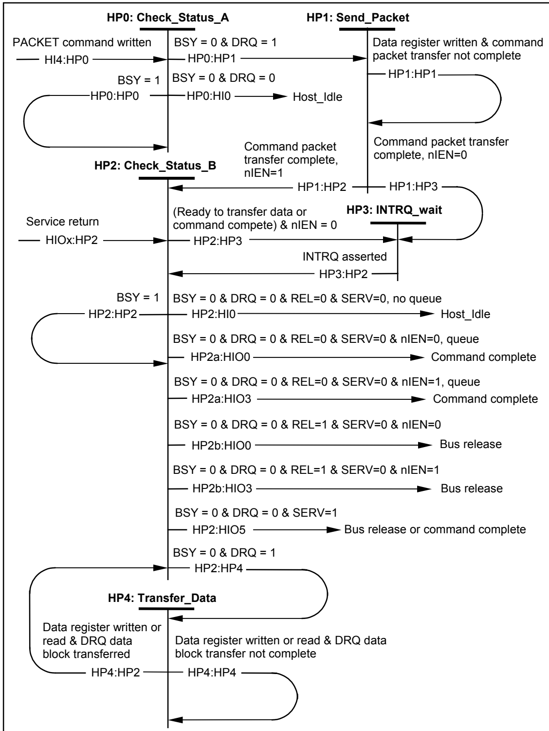
Figure 52 – Host PACKET non-data and PIO data command state diagram
