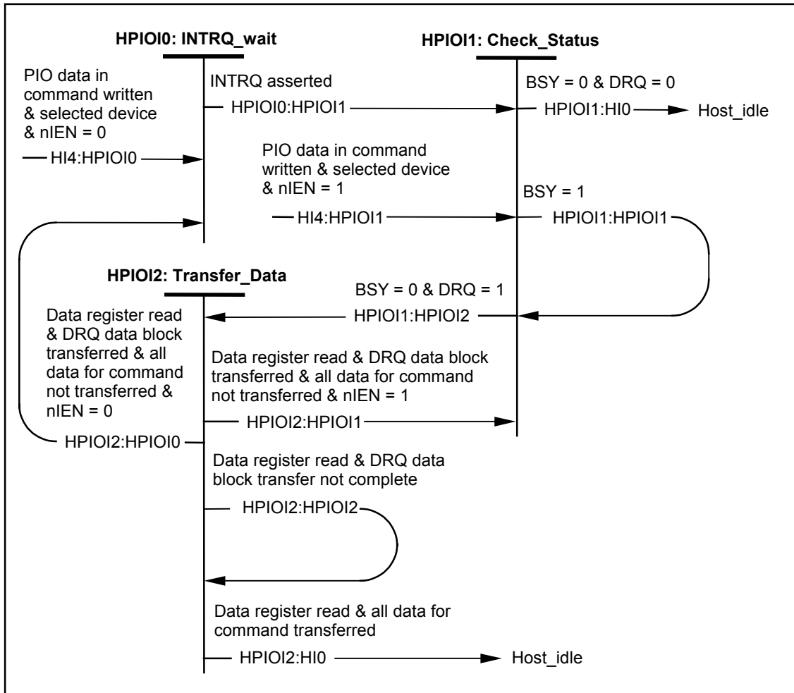
Figure 46 – Host PIO data-In state diagram
