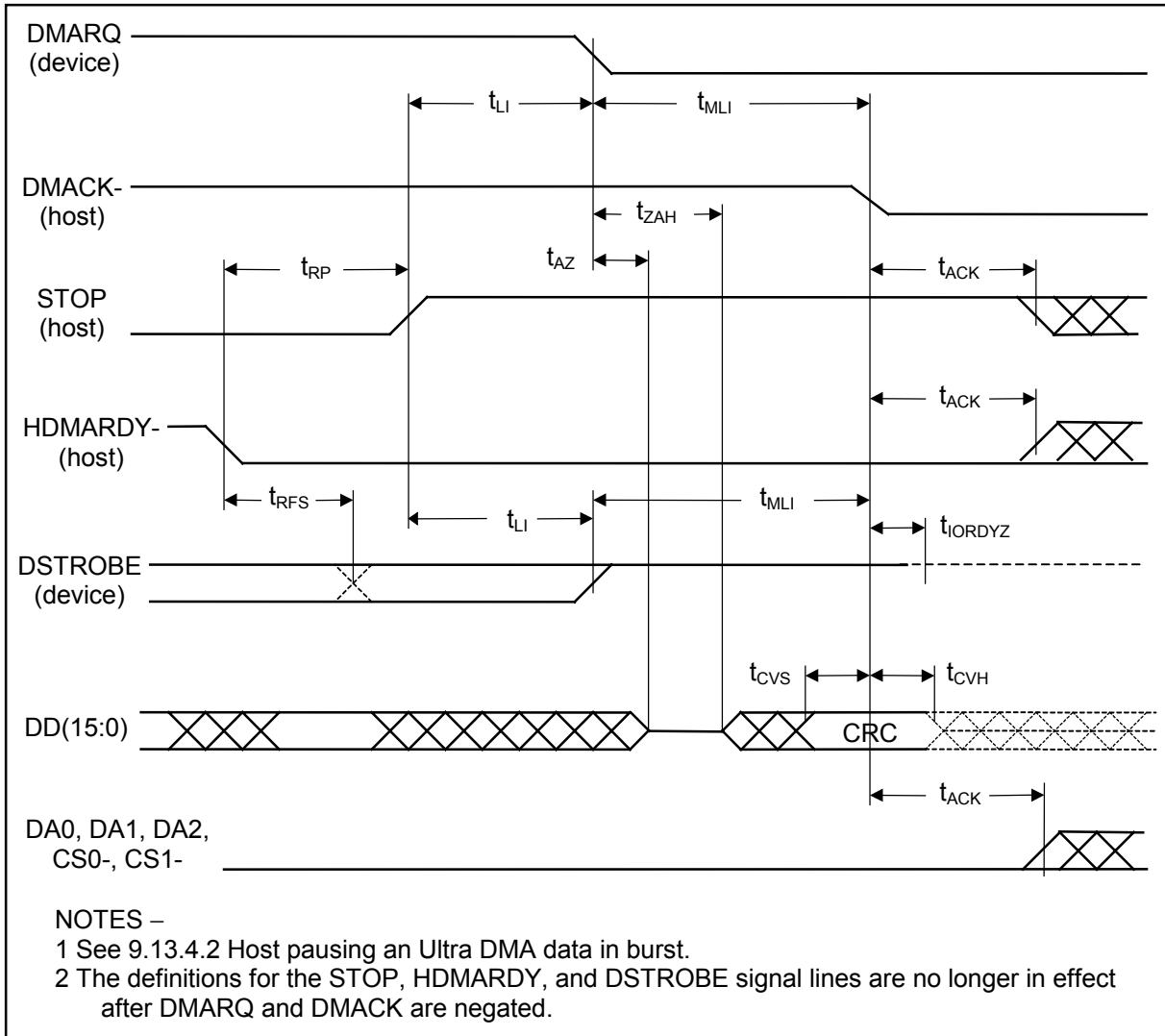
Figure 74 – Host terminating an Ultra DMA data-in burst
