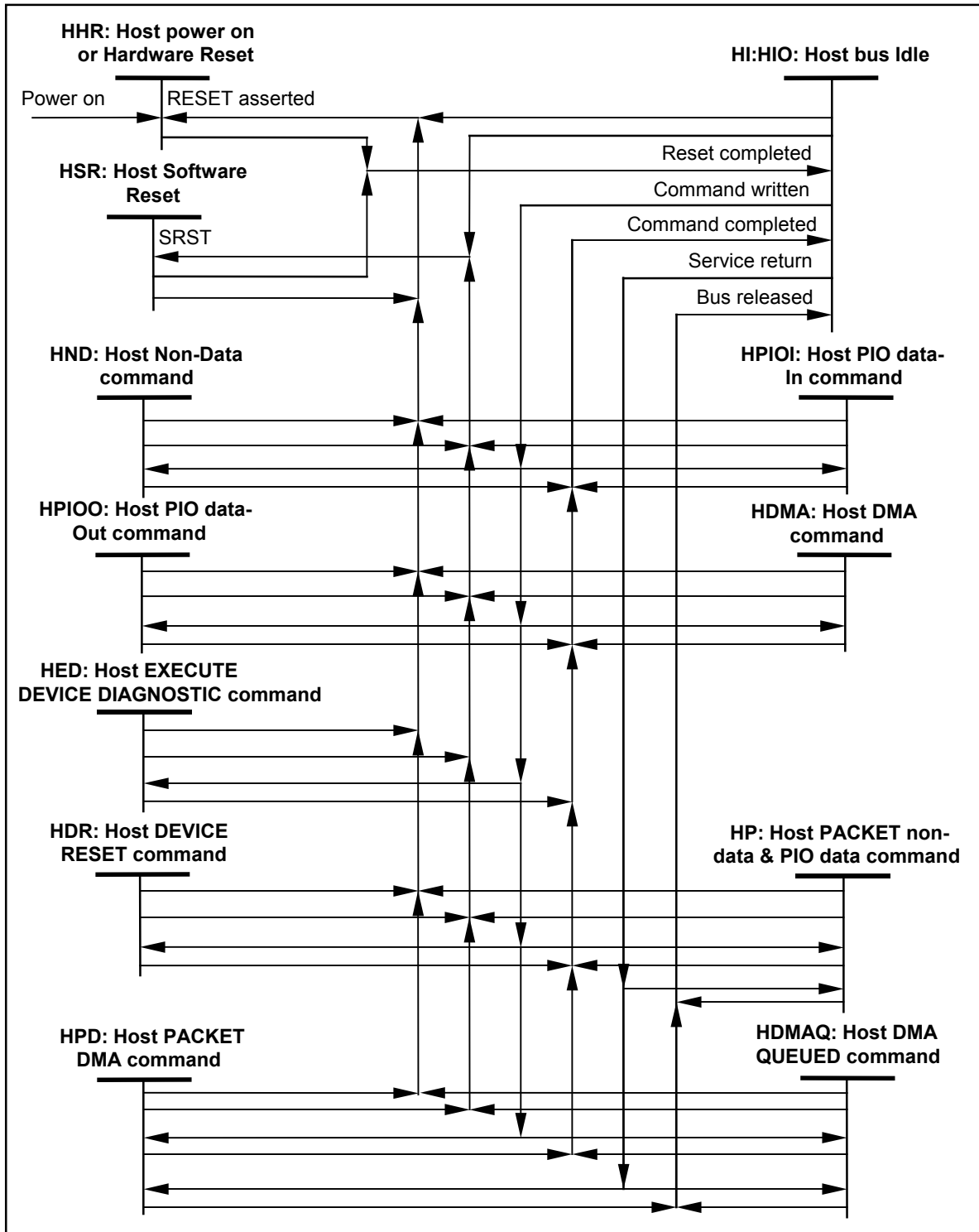
Figure 33 – Overall host protocol state sequence
