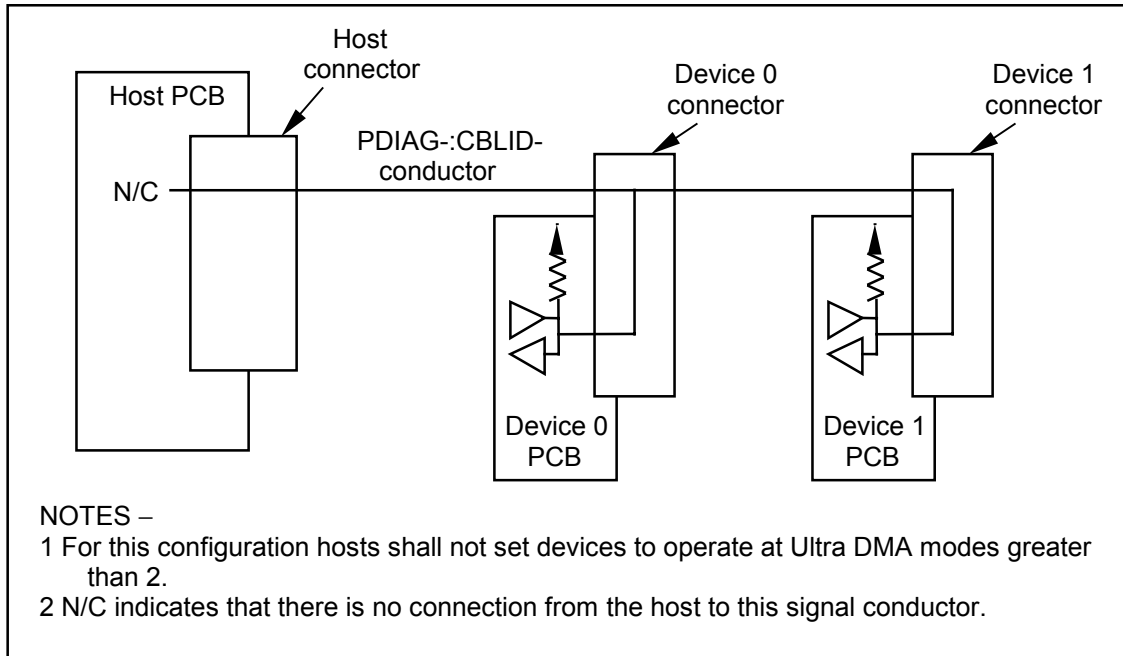
Figure 30 – Example configuration of a system with a 40-conductor cable
