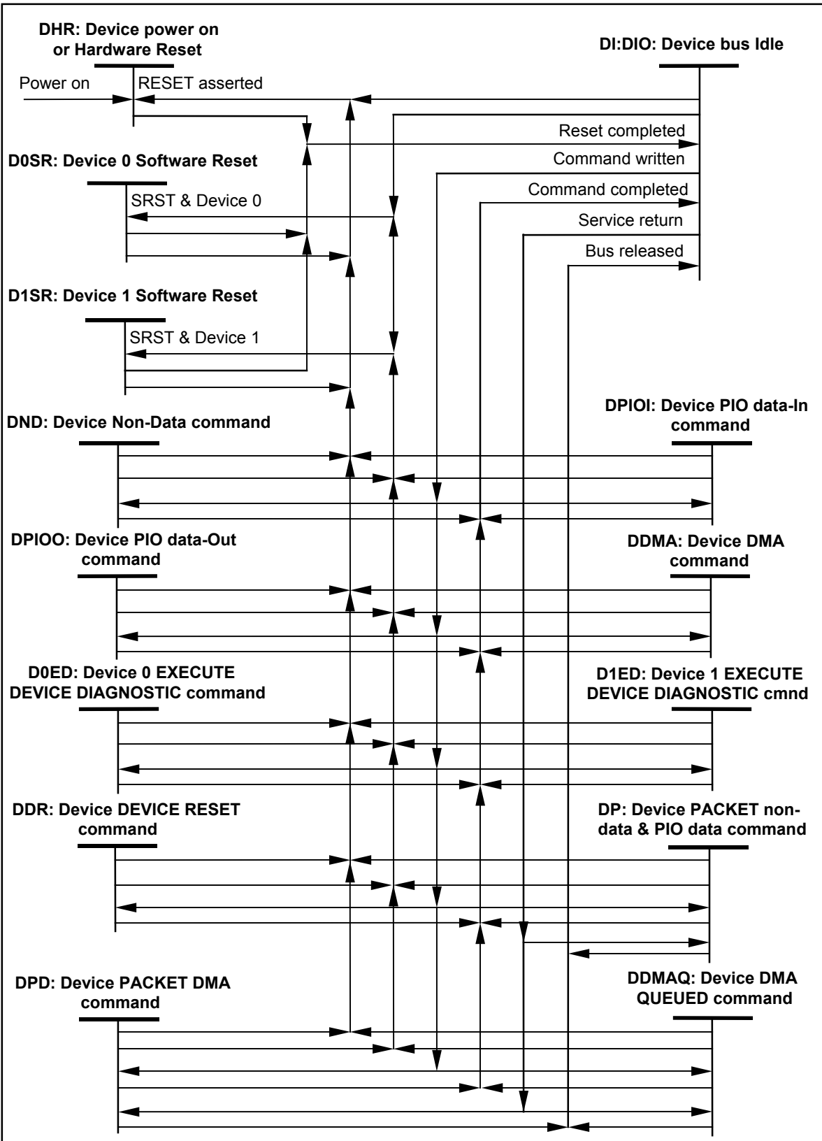
Figure 34 – Overall device protocol state sequence
