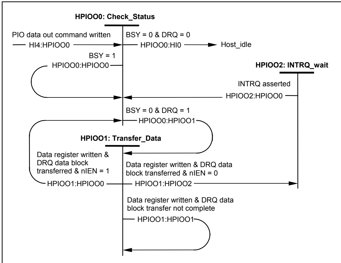
Figure 48 – Host PIO data-Out state diagram
