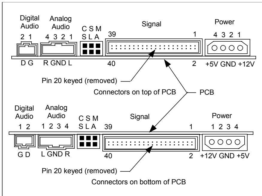
Figure 27 – 5.25 inch CD-ROM connector location
