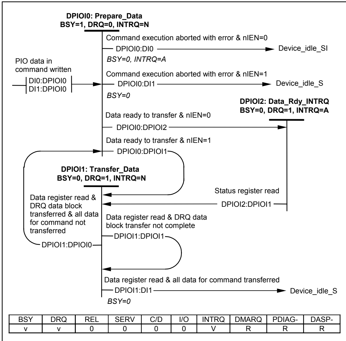
Figure 47 – Device PIO data-In state diagram
