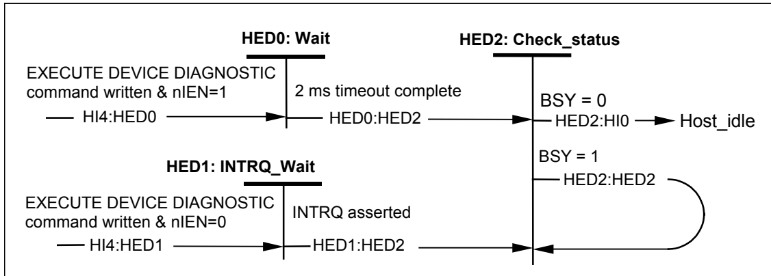
Figure 58 – Host EXECUTE DEVICE DIAGNOSTIC state diagram
