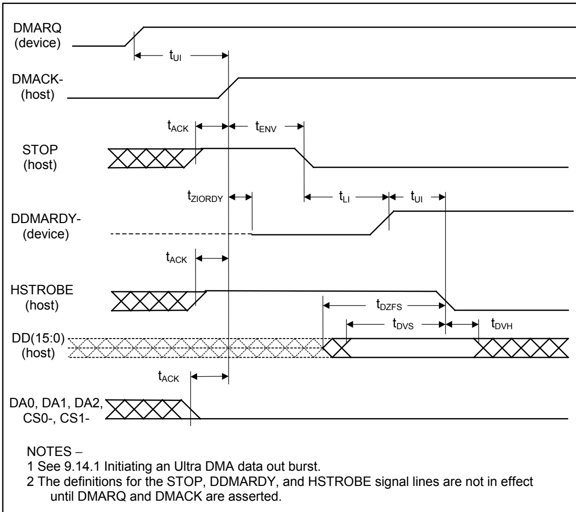
Figure 75 – Initiating an Ultra DMA data-out burst
