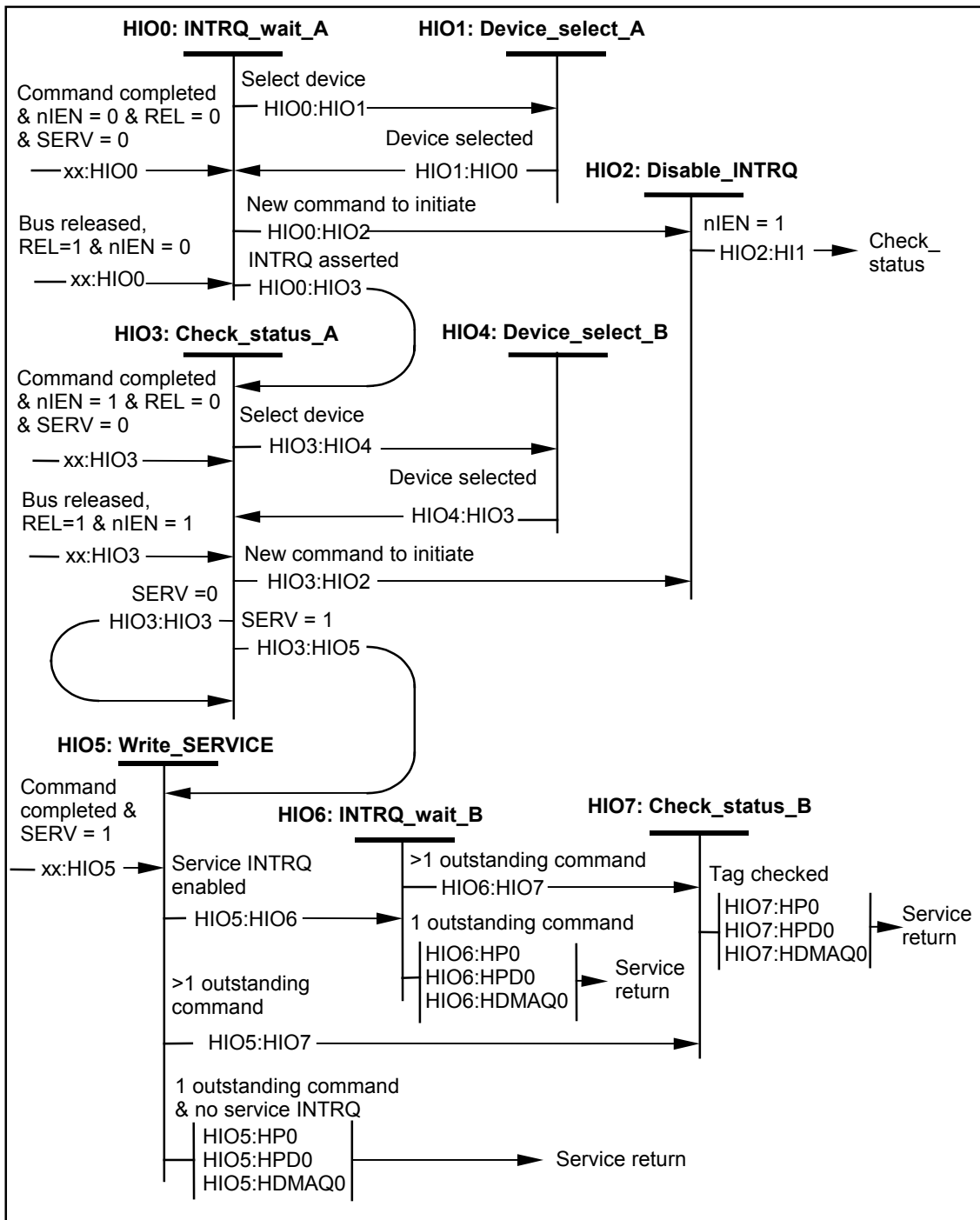
Figure 41 – Additional Host bus Idle state diagram with Overlap or overlap and queuing
