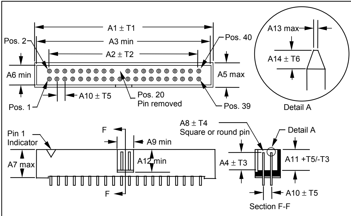
Figure 4 – Host or device 40-pin I/O header
