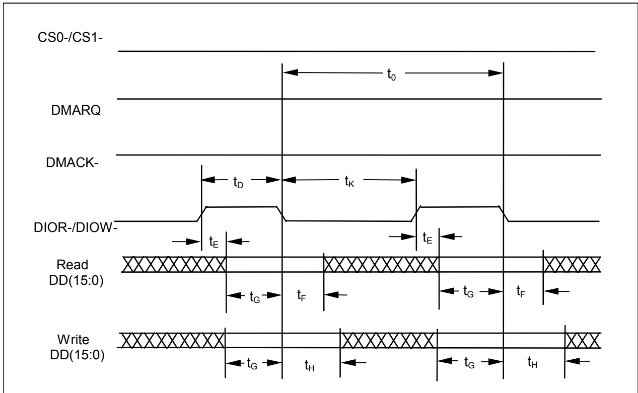
Figure 67 – Sustaining a Multiword DMA data burst
