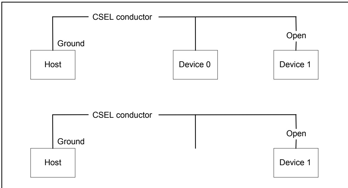
Figure 28 – Cable select example
