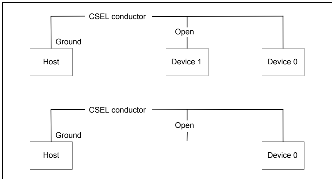
Figure 29 – Alternate cable select example
