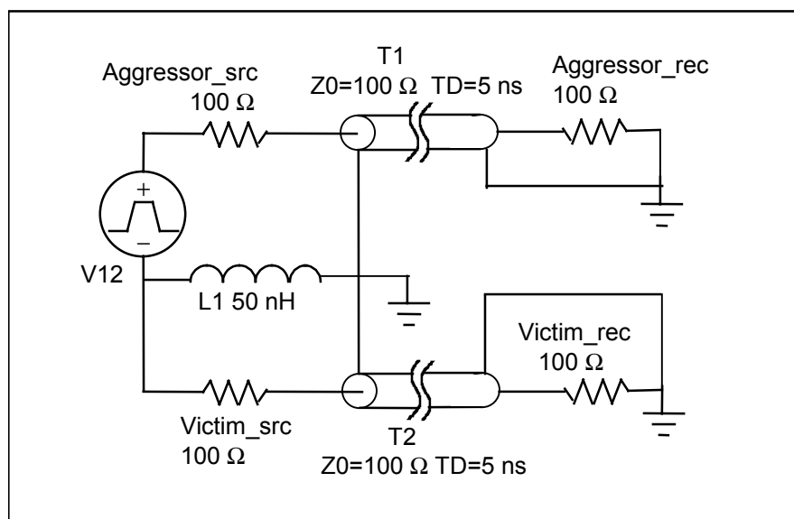
Figure E.20 – Model of ground bounce in IC package
