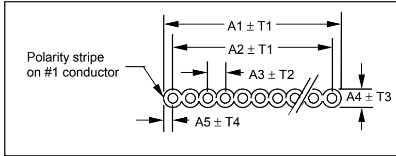
Figure 8 – 80-conductor ribbon cable
