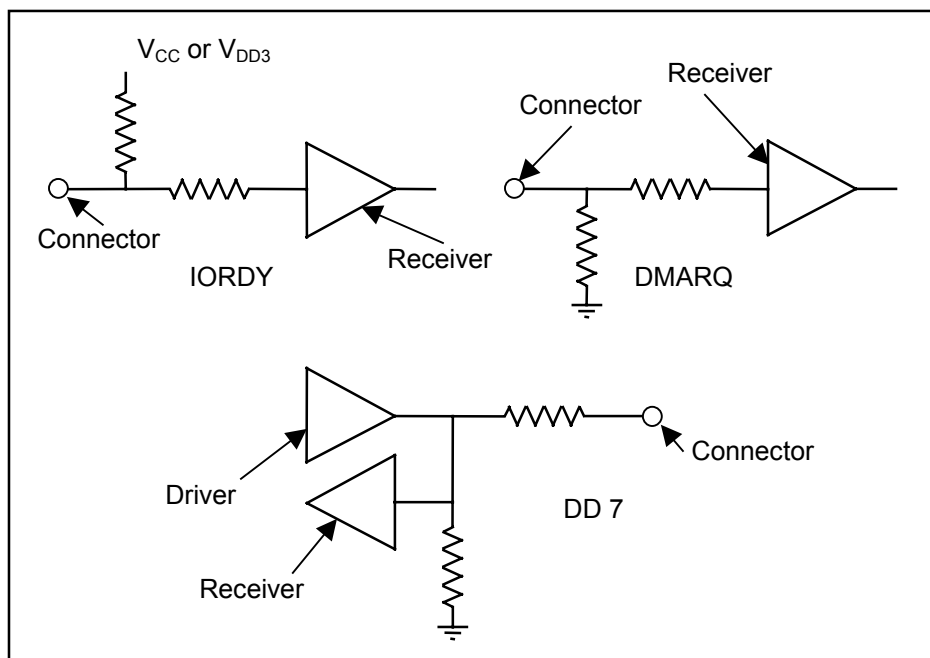
Figure 3 – Ultra DMA termination with pull-up or pull-down
