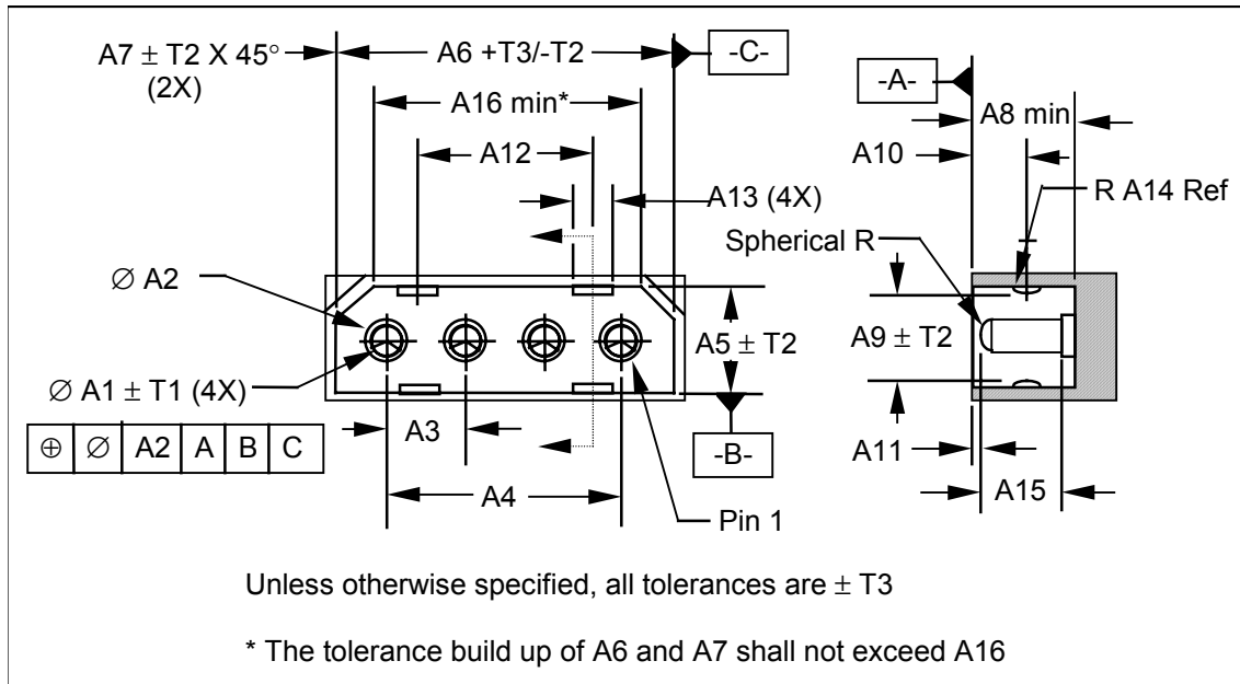
Figure 11 – Device 4-pin power header
