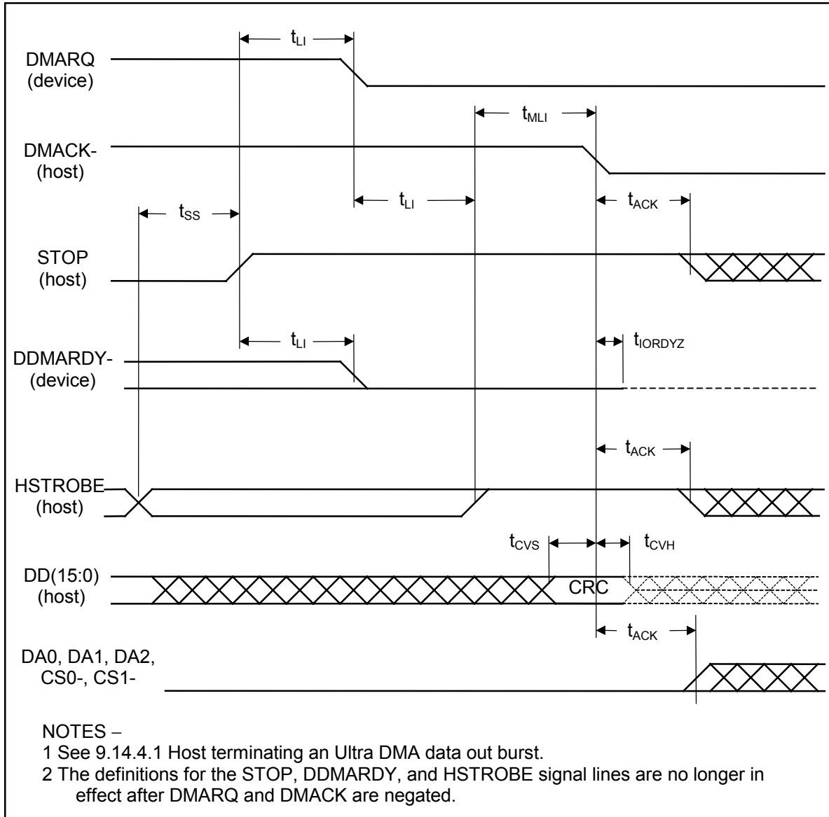
Figure 78 – Host terminating an Ultra DMA data-out burst
