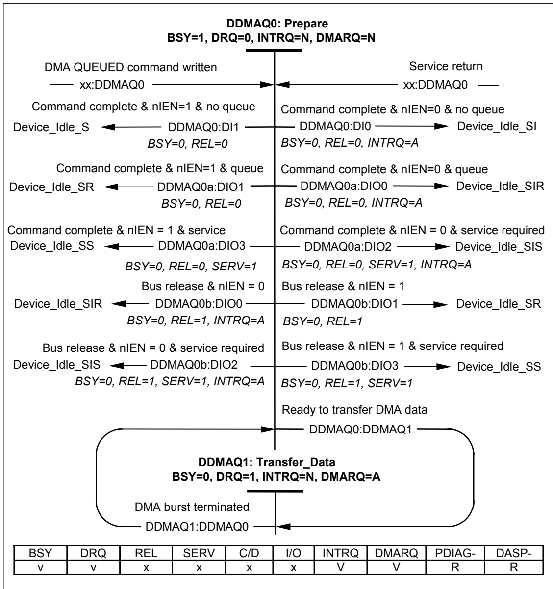
Figure 57 – Device DMA QUEUED command state diagram
