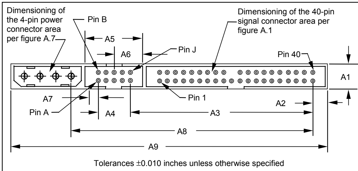
Figure 14 – Unitized connector
