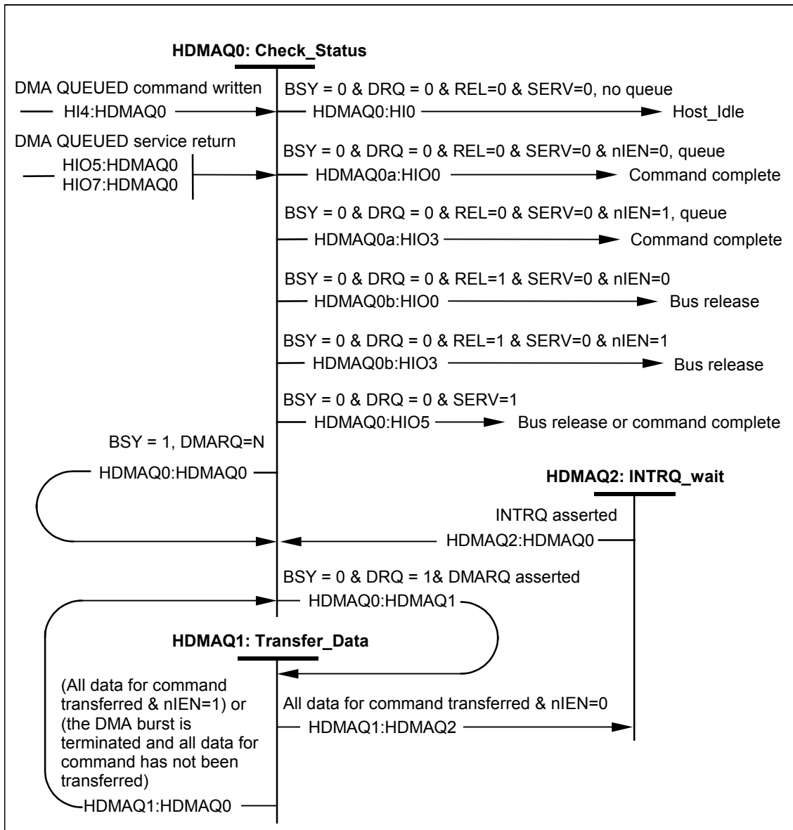
Figure 56 – Host DMA QUEUED state diagram
