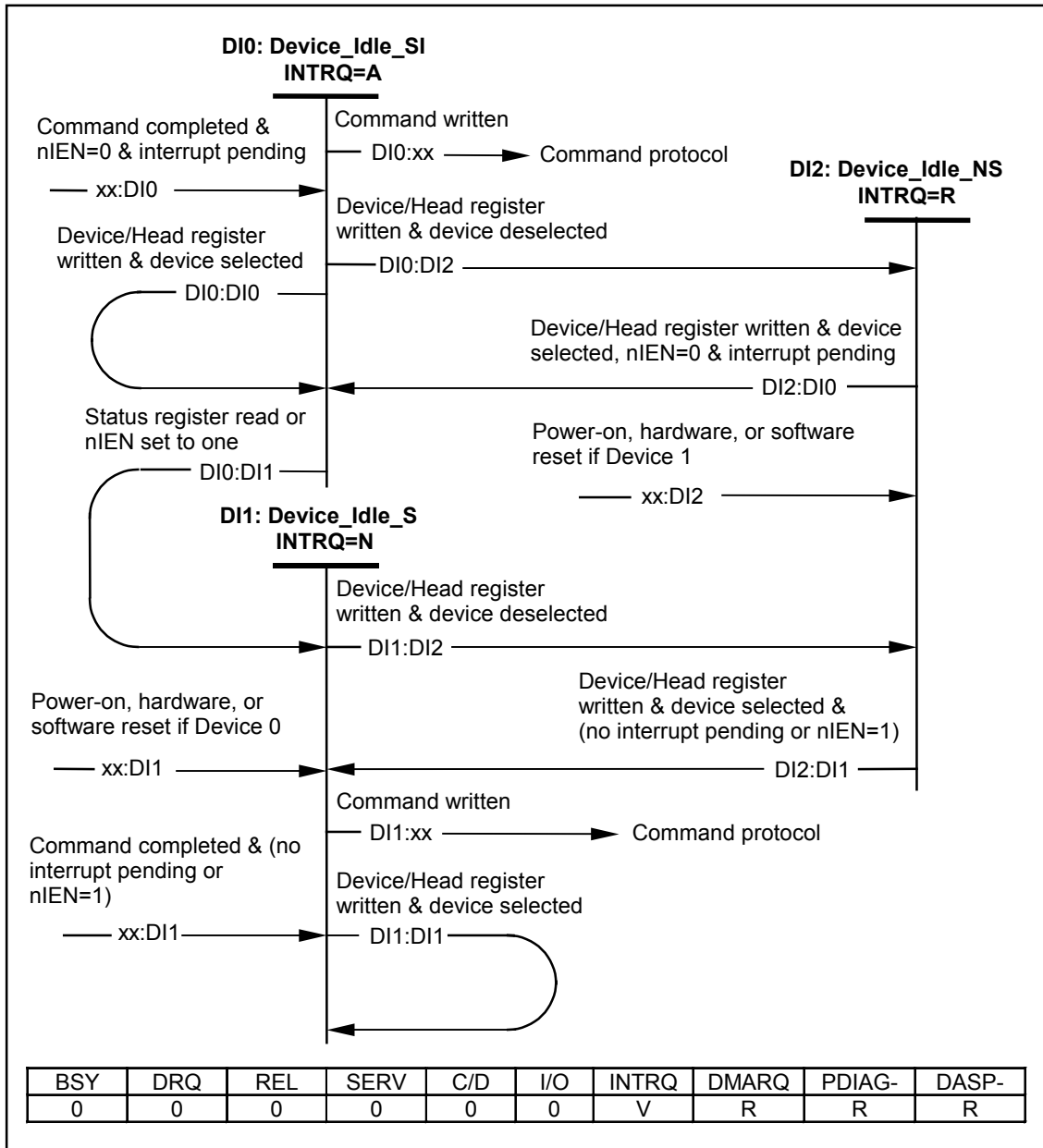
Figure 42 – Device bus Idle state diagram
